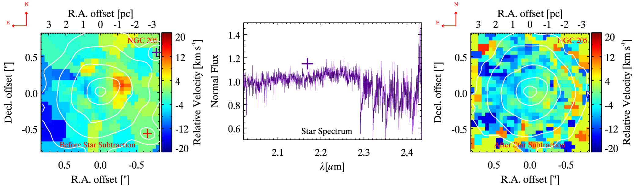
Figure 4. from Nearby Early-type Galactic Nuclei at High Resolution: Dynamical Black Hole and Nuclear Star Cluster Mass Measurements null 2018 APJ 858 118 doi:10.3847/1538-4357/aabe28 https://dx.doi.org/10.3847/1538-4357/aabe28 © 2018. The American Astronomical Society. All rights reserved.
