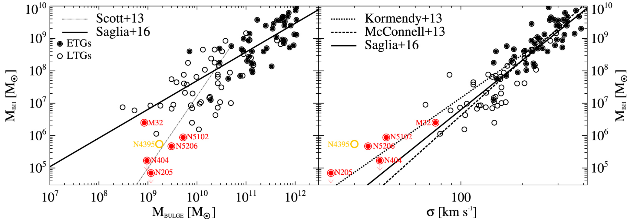
Figure 10. from Nearby Early-type Galactic Nuclei at High Resolution: Dynamical Black Hole and Nuclear Star Cluster Mass Measurements null 2018 APJ 858 118 doi:10.3847/1538-4357/aabe28 https://dx.doi.org/10.3847/1538-4357/aabe28 © 2018. The American Astronomical Society. All rights reserved.
