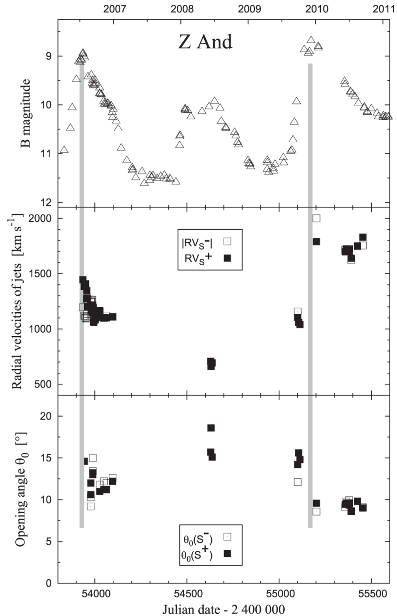
Figure 6. from Repeated Transient Jets from a Warped Disk in the Symbiotic Prototype Z And: A Link to the Long-lasting Active Phase null 2018 APJ 858 120 doi:10.3847/1538-4357/aabc11 https://dx.doi.org/10.3847/1538-4357/aabc11 © 2018. The American Astronomical Society. All rights reserved.
