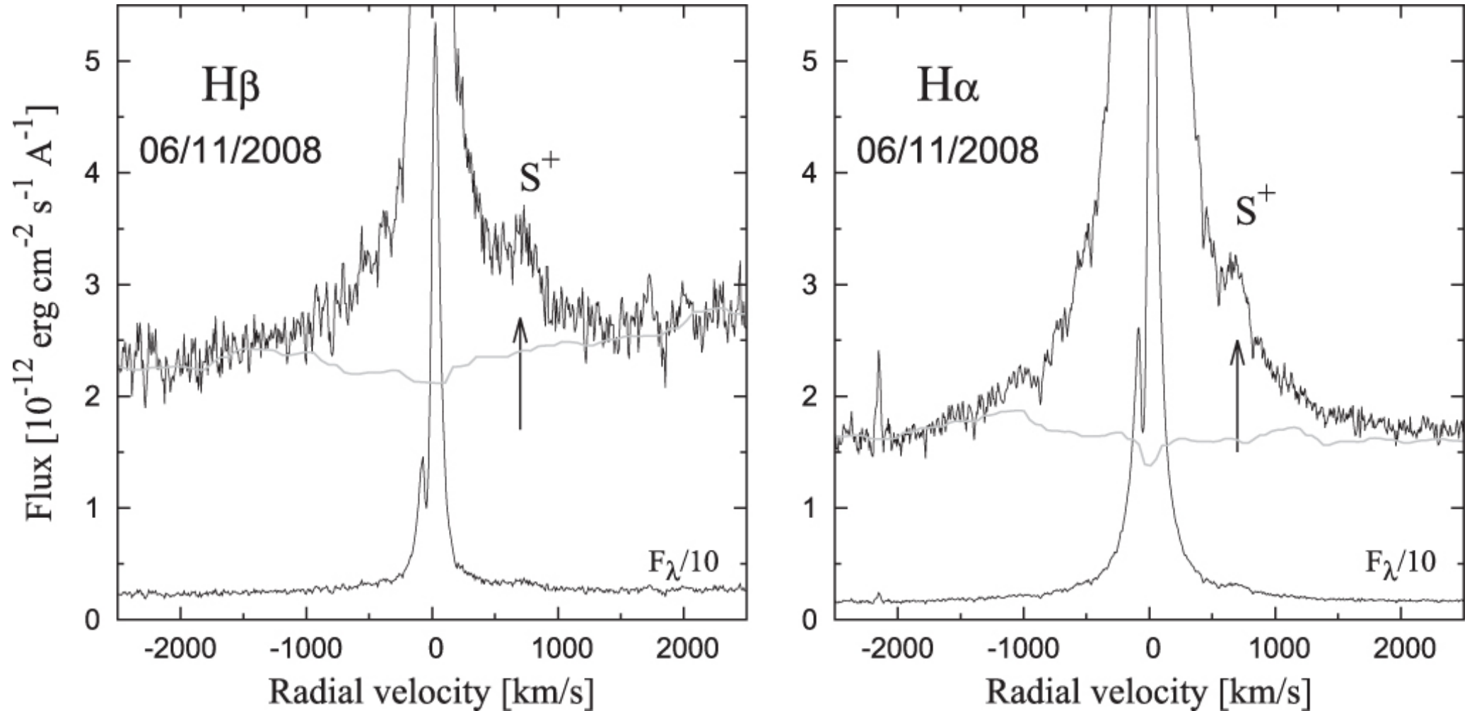
Figure 2. from Repeated Transient Jets from a Warped Disk in the Symbiotic Prototype Z And: A Link to the Long-lasting Active Phase null 2018 APJ 858 120 doi:10.3847/1538-4357/aabc11 https://dx.doi.org/10.3847/1538-4357/aabc11 © 2018. The American Astronomical Society. All rights reserved.
