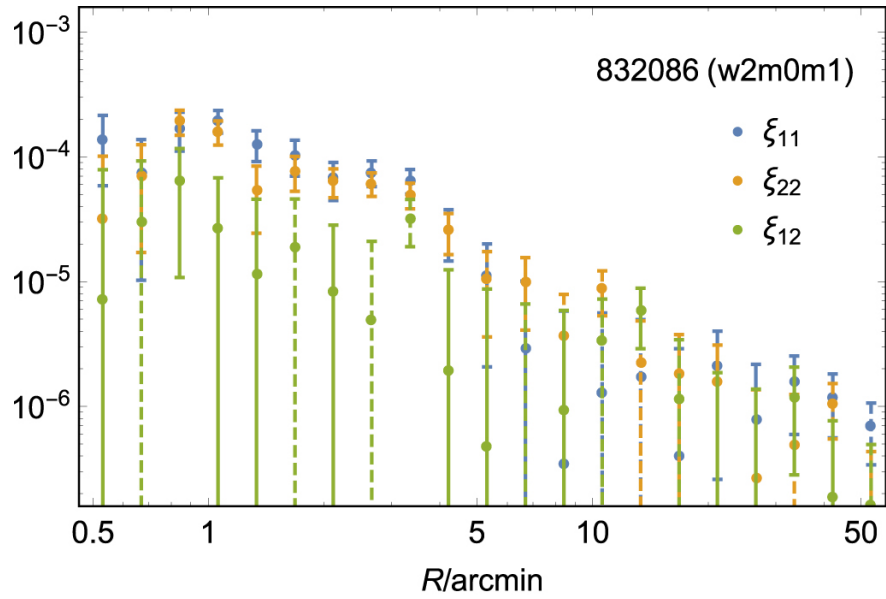
Figure 4. from Removing the Impact of Correlated PSF Uncertainties in Weak Lensing null 2018 APJ 858 122 doi:10.3847/1538-4357/aabb50 https://dx.doi.org/10.3847/1538-4357/aabb50 © 2018. The American Astronomical Society. All rights reserved.
