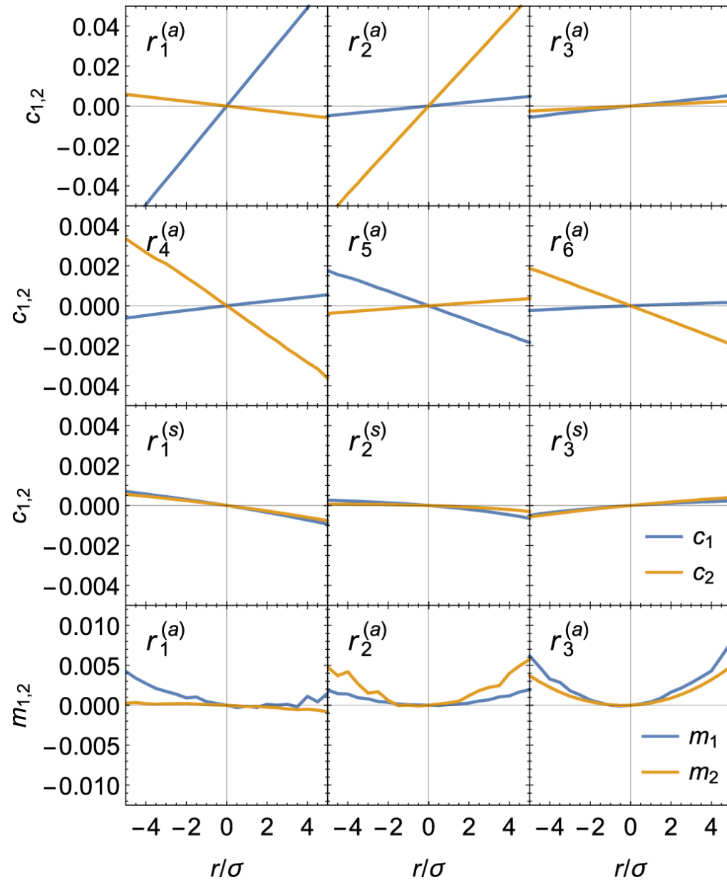
Figure 3. from Removing the Impact of Correlated PSF Uncertainties in Weak Lensing null 2018 APJ 858 122 doi:10.3847/1538-4357/aabb50 https://dx.doi.org/10.3847/1538-4357/aabb50 © 2018. The American Astronomical Society. All rights reserved.
