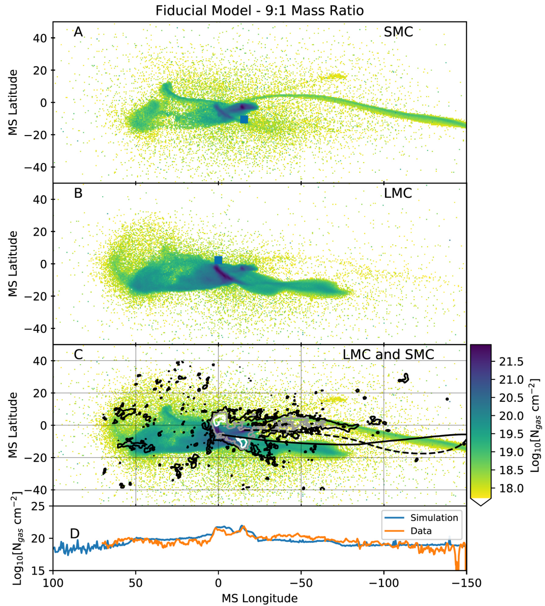
Figure 3. from Models of Tidally Induced Gas Filaments in the Magellanic Stream null 2018 APJ 857 101 doi:10.3847/1538-4357/aab95b https://dx.doi.org/10.3847/1538-4357/aab95b © 2018. The American Astronomical Society. All rights reserved.
