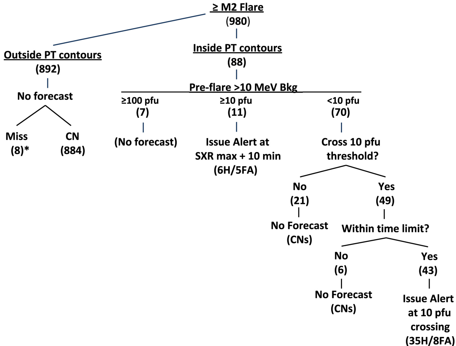
Figure 4. from A Short-term ESPERTA-based Forecast Tool for Moderate-to-extreme Solar Proton Events null 2018 APJ 857 107 doi:10.3847/1538-4357/aab712 https://dx.doi.org/10.3847/1538-4357/aab712 © 2018. The American Astronomical Society. All rights reserved.
