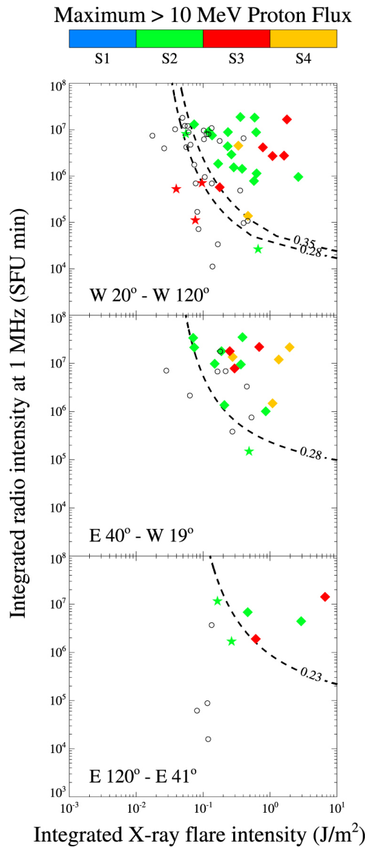
Figure 3. from A Short-term ESPERTA-based Forecast Tool for Moderate-to-extreme Solar Proton Events null 2018 APJ 857 107 doi:10.3847/1538-4357/aab712 https://dx.doi.org/10.3847/1538-4357/aab712 © 2018. The American Astronomical Society. All rights reserved.
