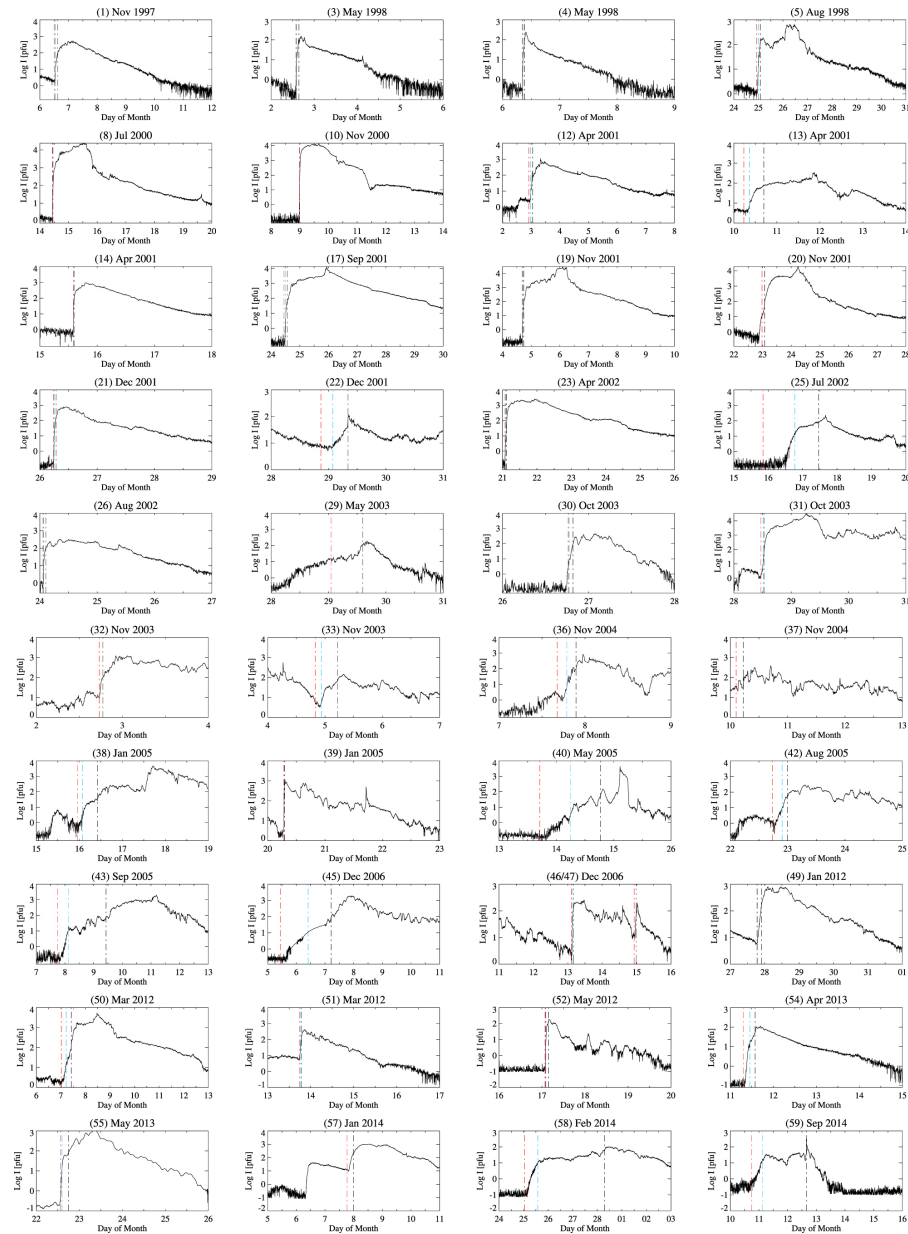
Figure 1. from A Short-term ESPERTA-based Forecast Tool for Moderate-to-extreme Solar Proton Events null 2018 APJ 857 107 doi:10.3847/1538-4357/aab712 https://dx.doi.org/10.3847/1538-4357/aab712 © 2018. The American Astronomical Society. All rights reserved.
