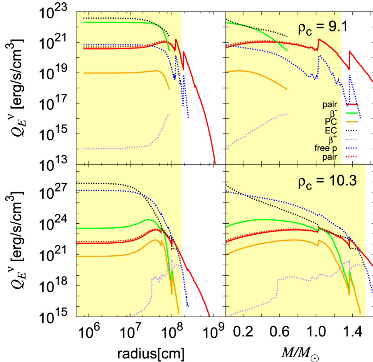
Figure 8. from Neutrino Emissions in All Flavors up to the Pre-bounce of Massive Stars and the Possibility of Their Detections null 2017 APJ 848 48 doi:10.3847/1538-4357/aa8b72 https://dx.doi.org/10.3847/1538-4357/aa8b72 © 2017. The American Astronomical Society. All rights reserved.
