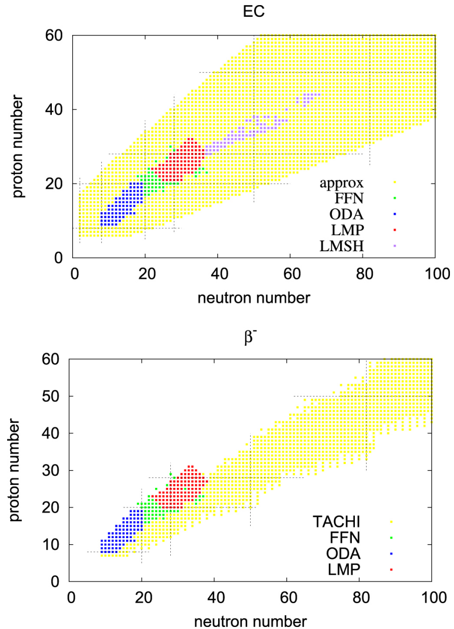
Figure 4. from Neutrino Emissions in All Flavors up to the Pre-bounce of Massive Stars and the Possibility of Their Detections null 2017 APJ 848 48 doi:10.3847/1538-4357/aa8b72 https://dx.doi.org/10.3847/1538-4357/aa8b72 © 2017. The American Astronomical Society. All rights reserved.
