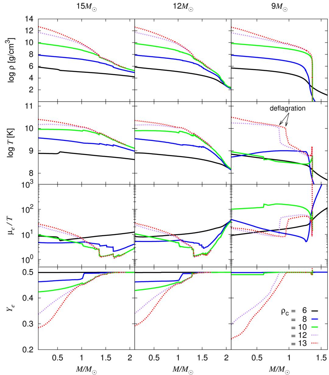
Figure 3. from Neutrino Emissions in All Flavors up to the Pre-bounce of Massive Stars and the Possibility of Their Detections null 2017 APJ 848 48 doi:10.3847/1538-4357/aa8b72 https://dx.doi.org/10.3847/1538-4357/aa8b72 © 2017. The American Astronomical Society. All rights reserved.
