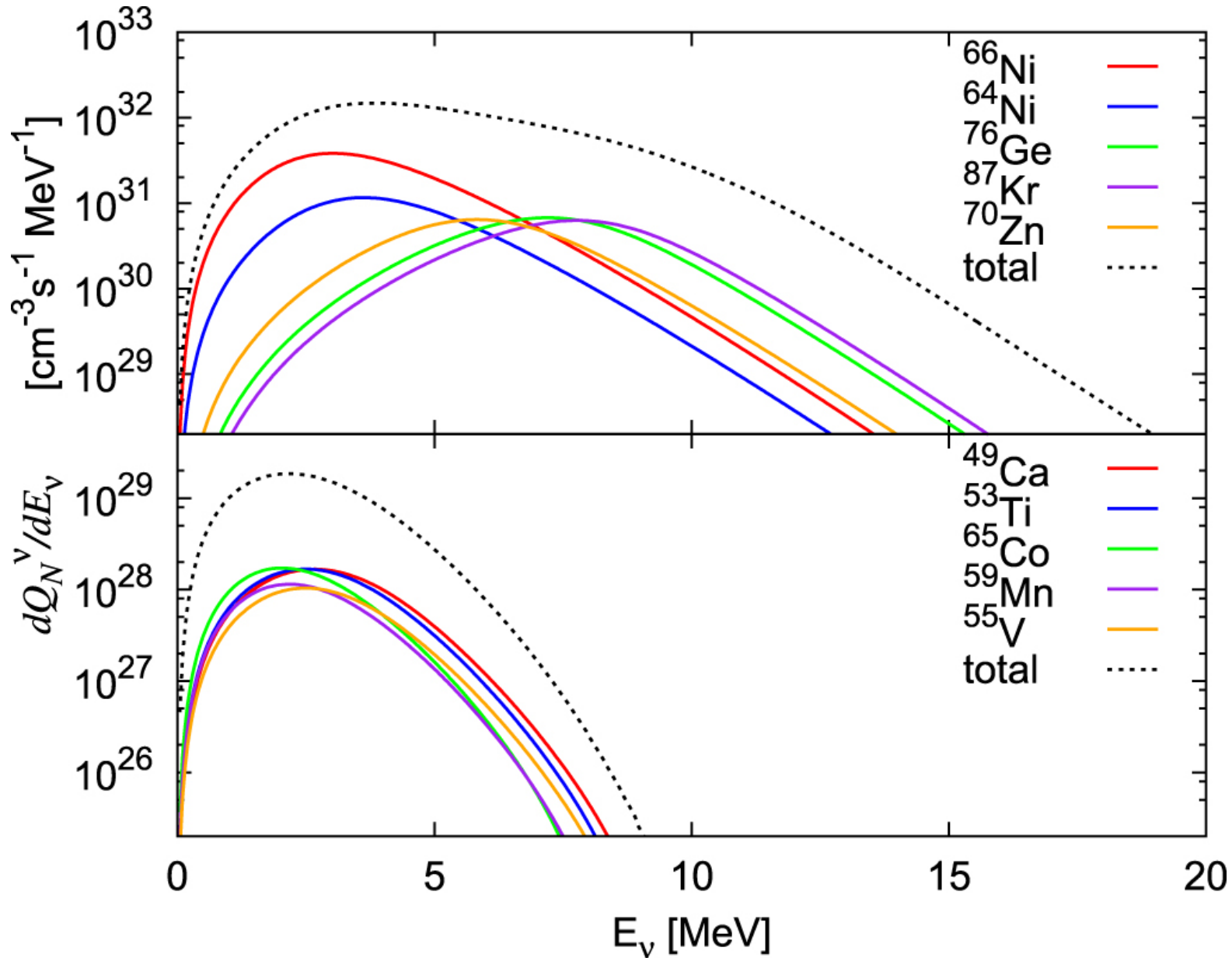
Figure 10. from Neutrino Emissions in All Flavors up to the Pre-bounce of Massive Stars and the Possibility of Their Detections null 2017 APJ 848 48 doi:10.3847/1538-4357/aa8b72 https://dx.doi.org/10.3847/1538-4357/aa8b72 © 2017. The American Astronomical Society. All rights reserved.
