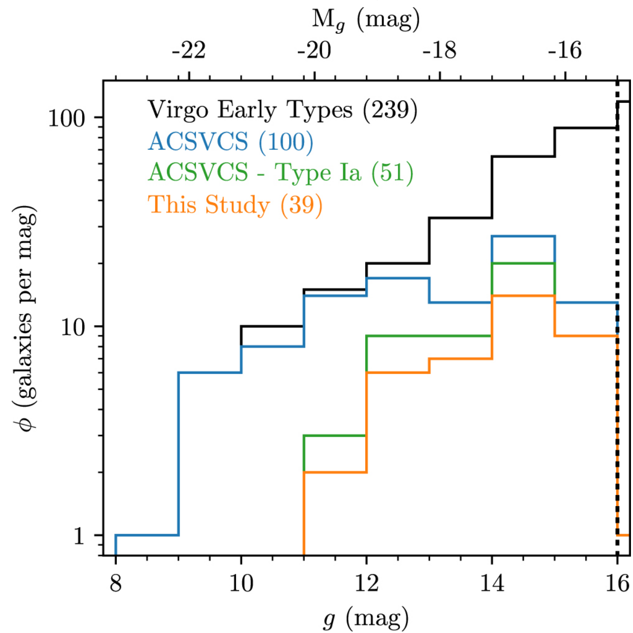
Figure 4. from Virgo Redux: The Masses and Stellar Content of Nuclei in Early-type Galaxies from Multiband Photometry and Spectroscopy null 2017 APJ 849 55 doi:10.3847/1538-4357/aa8a78 https://dx.doi.org/10.3847/1538-4357/aa8a78 © 2017. The American Astronomical Society. All rights reserved.
