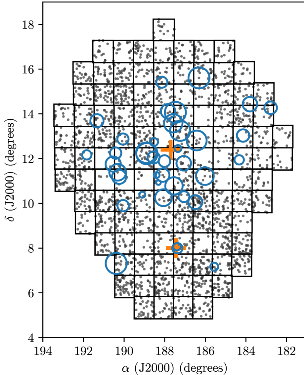
Figure 3. from Virgo Redux: The Masses and Stellar Content of Nuclei in Early-type Galaxies from Multiband Photometry and Spectroscopy null 2017 APJ 849 55 doi:10.3847/1538-4357/aa8a78 https://dx.doi.org/10.3847/1538-4357/aa8a78 © 2017. The American Astronomical Society. All rights reserved.
