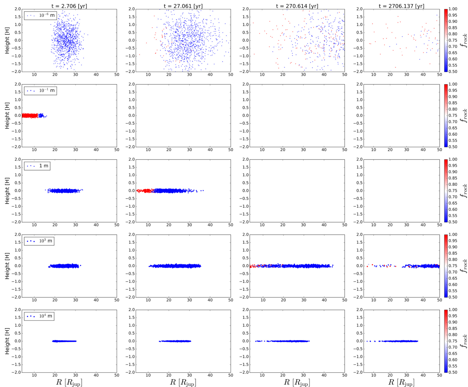
Figure 4. from Pebble Accretion at the Origin of Water in Europa null 2017 APJ 845 92 doi:10.3847/1538-4357/aa80e6 https://dx.doi.org/10.3847/1538-4357/aa80e6 © 2017. The American Astronomical Society. All rights reserved.
