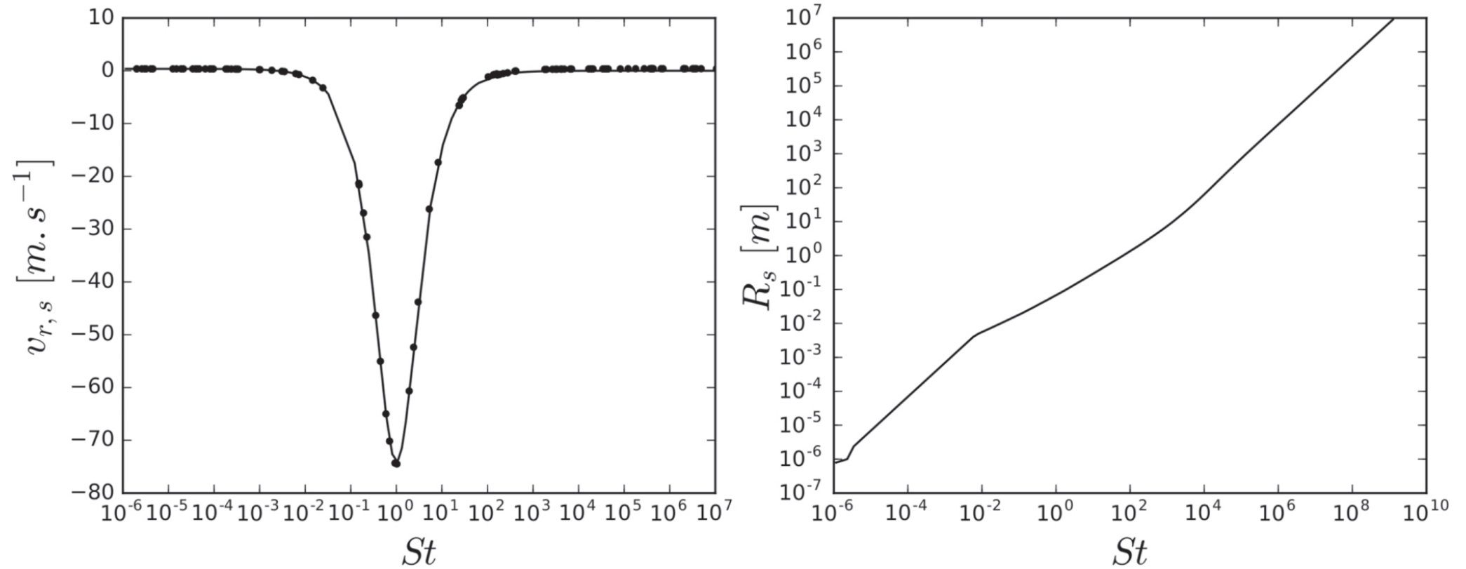
Figure 3. from Pebble Accretion at the Origin of Water in Europa null 2017 APJ 845 92 doi:10.3847/1538-4357/aa80e6 https://dx.doi.org/10.3847/1538-4357/aa80e6 © 2017. The American Astronomical Society. All rights reserved.
