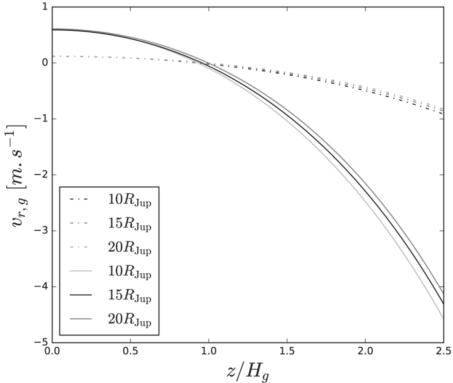
Figure 2. from Pebble Accretion at the Origin of Water in Europa null 2017 APJ 845 92 doi:10.3847/1538-4357/aa80e6 https://dx.doi.org/10.3847/1538-4357/aa80e6 © 2017. The American Astronomical Society. All rights reserved.
