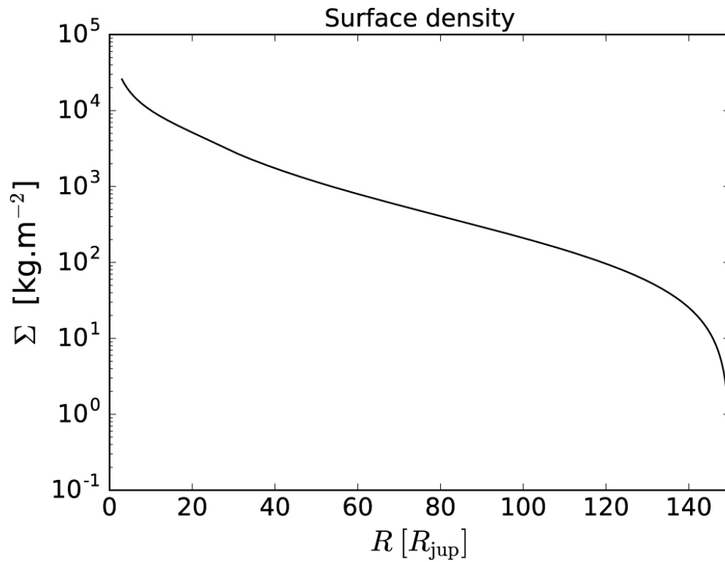
Figure 1. from Pebble Accretion at the Origin of Water in Europa null 2017 APJ 845 92 doi:10.3847/1538-4357/aa80e6 https://dx.doi.org/10.3847/1538-4357/aa80e6 © 2017. The American Astronomical Society. All rights reserved.
