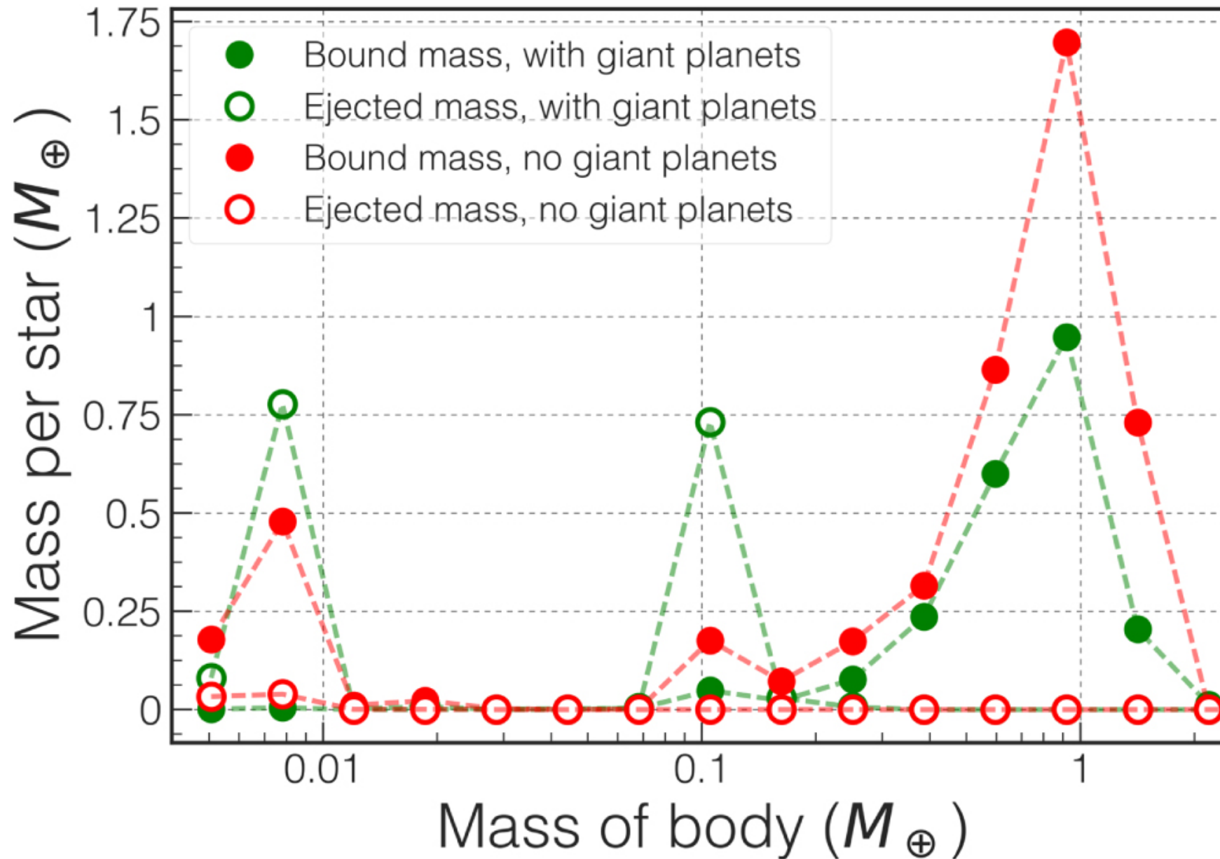
Figure 6. from The Demographics of Rocky Free-floating Planets and their Detectability by WFIRST null 2017 APJ 841 86 doi:10.3847/1538-4357/aa705b https://dx.doi.org/10.3847/1538-4357/aa705b © 2017. The American Astronomical Society. All rights reserved.
