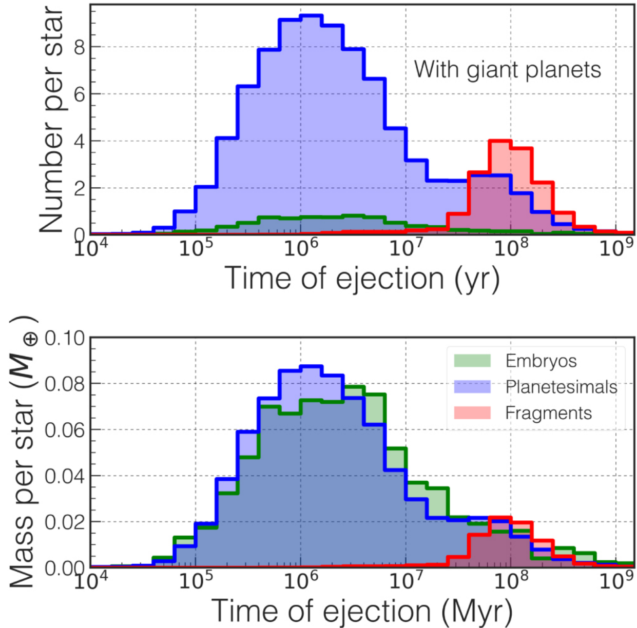
Figure 3. from The Demographics of Rocky Free-floating Planets and their Detectability by WFIRST null 2017 APJ 841 86 doi:10.3847/1538-4357/aa705b https://dx.doi.org/10.3847/1538-4357/aa705b © 2017. The American Astronomical Society. All rights reserved.
