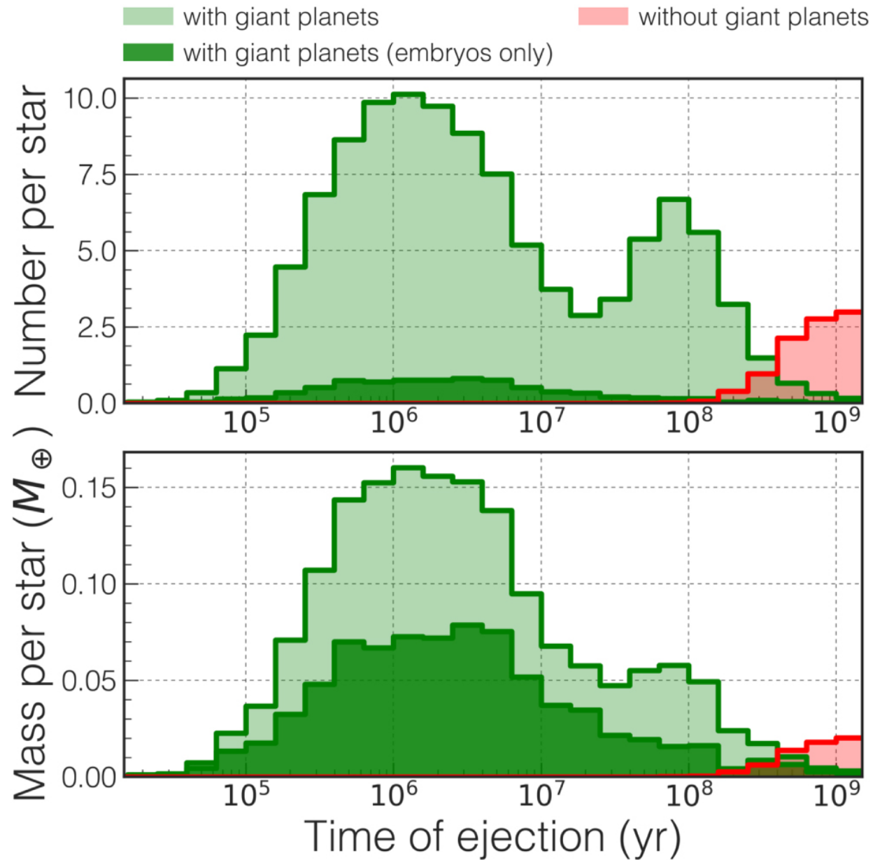
Figure 2. from The Demographics of Rocky Free-floating Planets and their Detectability by WFIRST null 2017 APJ 841 86 doi:10.3847/1538-4357/aa705b https://dx.doi.org/10.3847/1538-4357/aa705b © 2017. The American Astronomical Society. All rights reserved.
