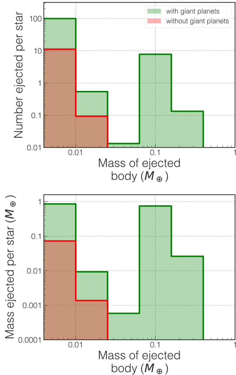
Figure 1. from The Demographics of Rocky Free-floating Planets and their Detectability by WFIRST null 2017 APJ 841 86 doi:10.3847/1538-4357/aa705b https://dx.doi.org/10.3847/1538-4357/aa705b © 2017. The American Astronomical Society. All rights reserved.
