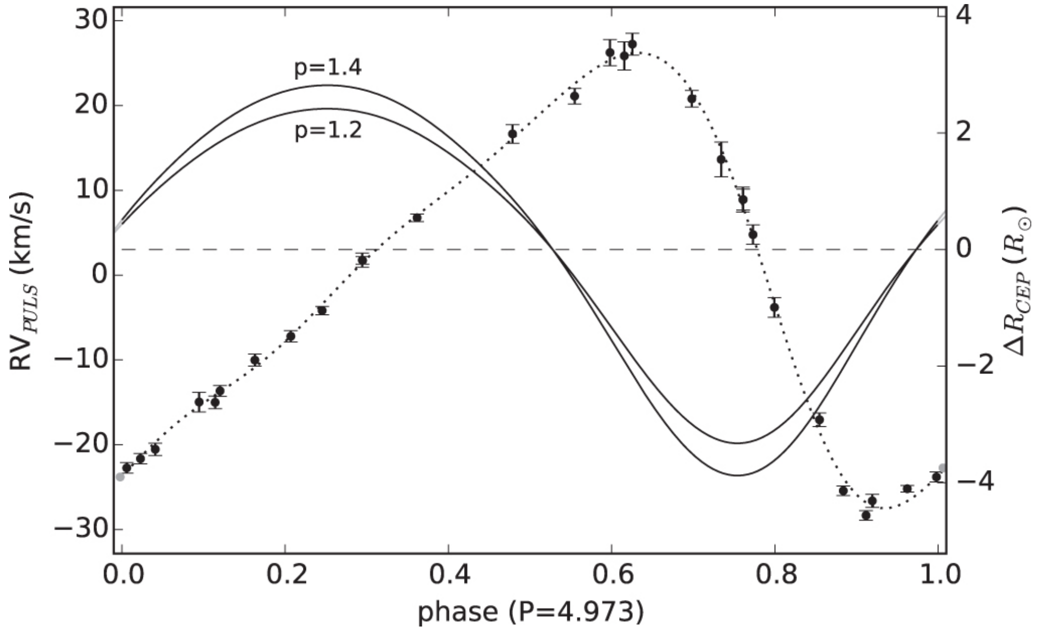
Figure 9. from Mass and p-factor of the Type II Cepheid OGLE-LMC-T2CEP-098 in a Binary System null 2017 APJ 842 110 doi:10.3847/1538-4357/aa6ff7 https://dx.doi.org/10.3847/1538-4357/aa6ff7 © 2017. The American Astronomical Society. All rights reserved.
