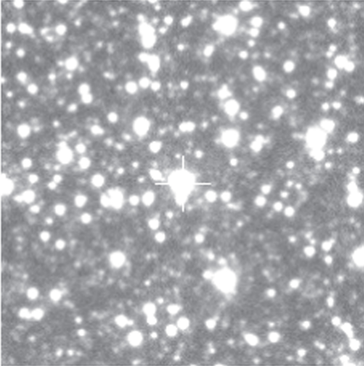
Figure 7. from Mass and p-factor of the Type II Cepheid OGLE-LMC-T2CEP-098 in a Binary System null 2017 APJ 842 110 doi:10.3847/1538-4357/aa6ff7 https://dx.doi.org/10.3847/1538-4357/aa6ff7 © 2017. The American Astronomical Society. All rights reserved.
