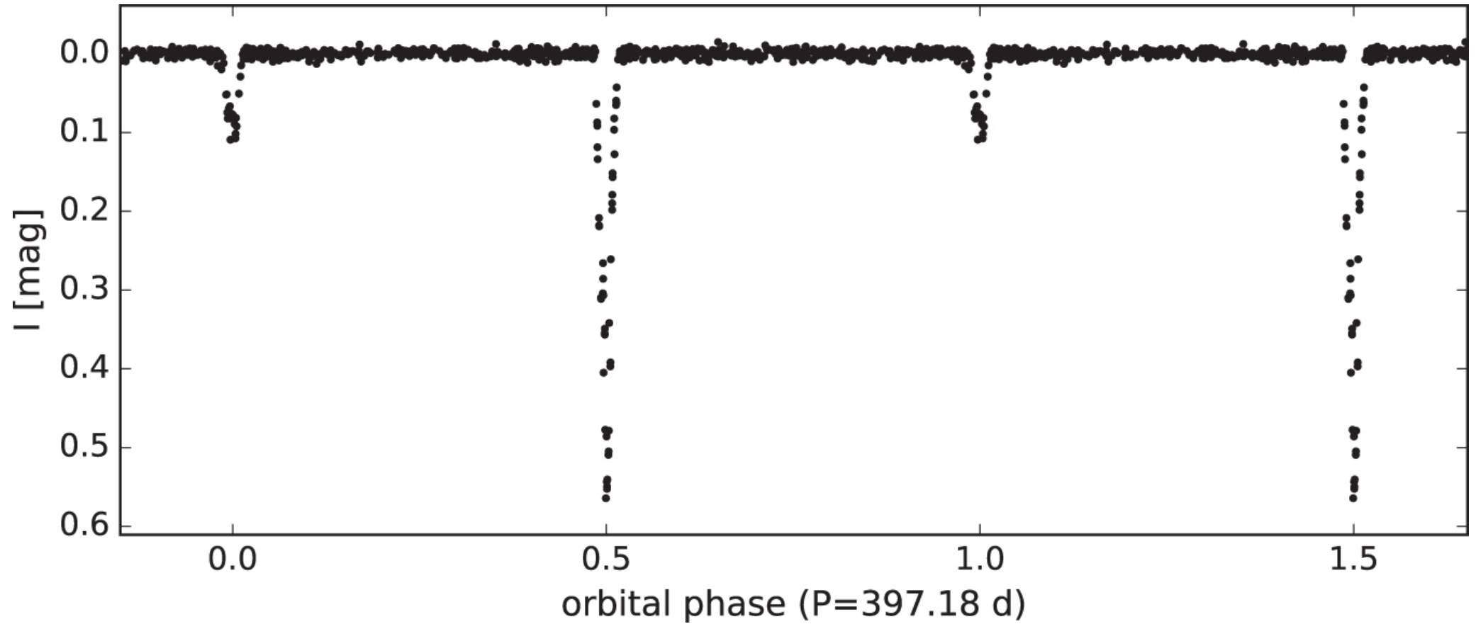
Figure 5. from Mass and p-factor of the Type II Cepheid OGLE-LMC-T2CEP-098 in a Binary System null 2017 APJ 842 110 doi:10.3847/1538-4357/aa6ff7 https://dx.doi.org/10.3847/1538-4357/aa6ff7 © 2017. The American Astronomical Society. All rights reserved.
