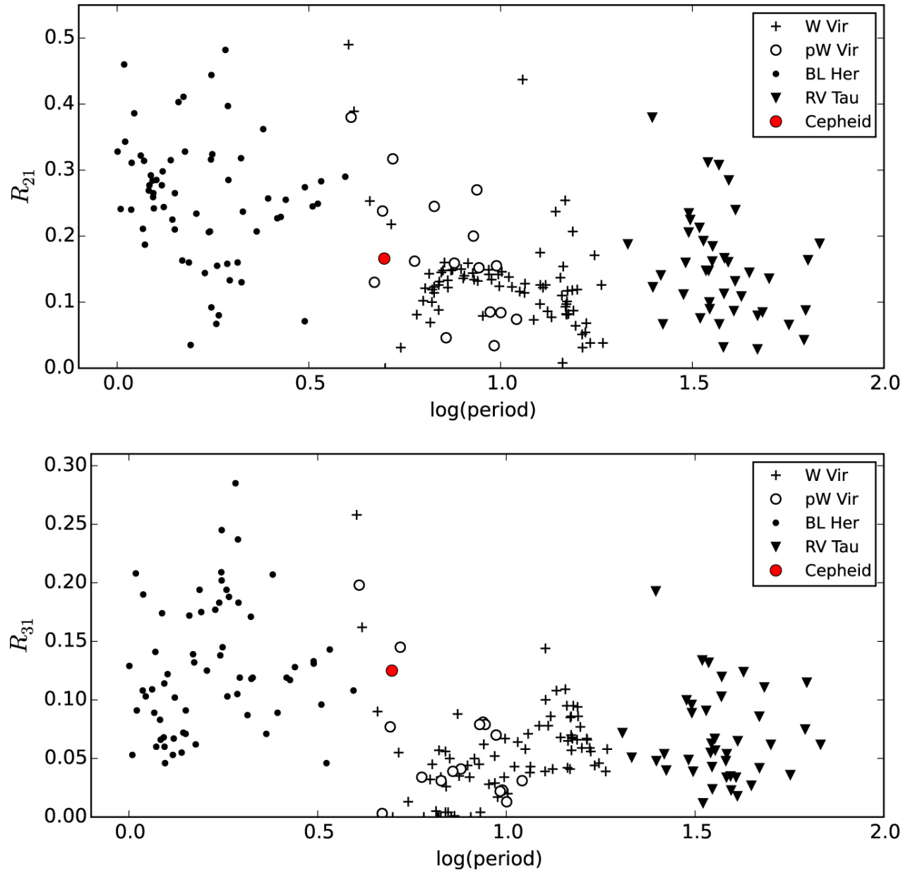
Figure 3. from Mass and p-factor of the Type II Cepheid OGLE-LMC-T2CEP-098 in a Binary System null 2017 APJ 842 110 doi:10.3847/1538-4357/aa6ff7 https://dx.doi.org/10.3847/1538-4357/aa6ff7 © 2017. The American Astronomical Society. All rights reserved.
