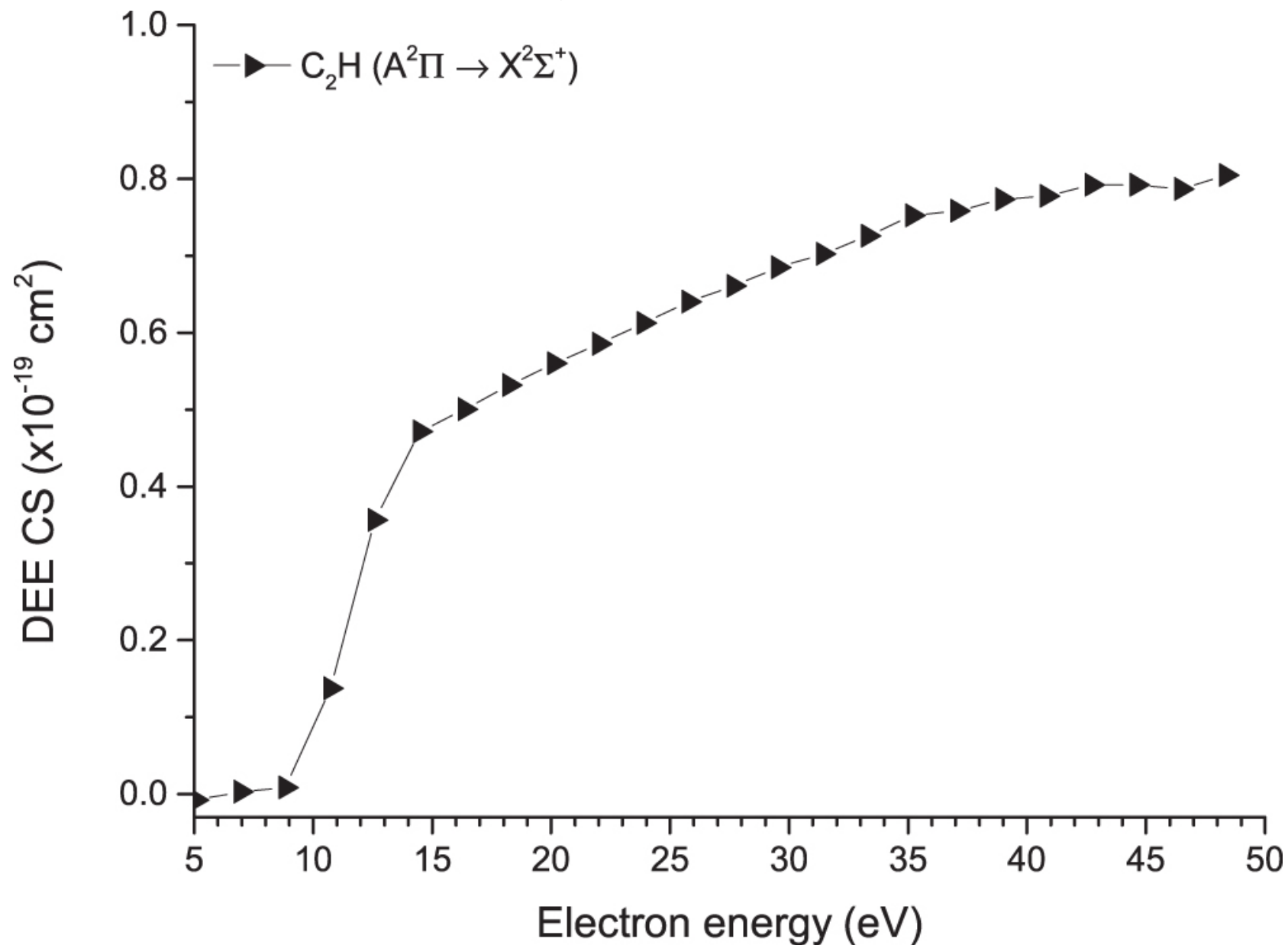
Figure 7. from Dissociative Excitation of Acetylene Induced by Electron Impact: Excitation-emission Cross-sections null 2017 APJ 841 17 doi:10.3847/1538-4357/aa6e54 https://dx.doi.org/10.3847/1538-4357/aa6e54 © 2017. The American Astronomical Society. All rights reserved.
