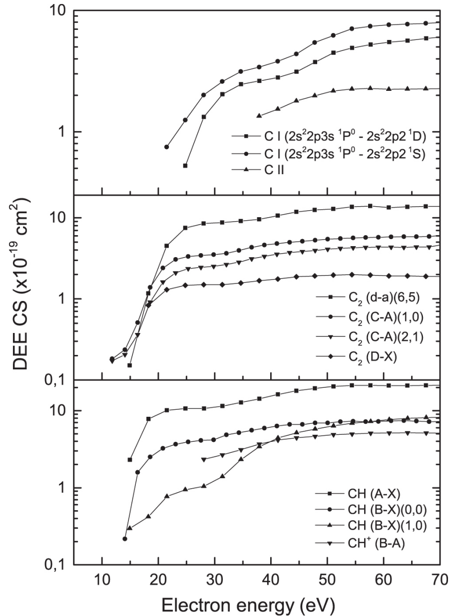
Figure 6. from Dissociative Excitation of Acetylene Induced by Electron Impact: Excitation-emission Cross-sections null 2017 APJ 841 17 doi:10.3847/1538-4357/aa6e54 https://dx.doi.org/10.3847/1538-4357/aa6e54 © 2017. The American Astronomical Society. All rights reserved.
