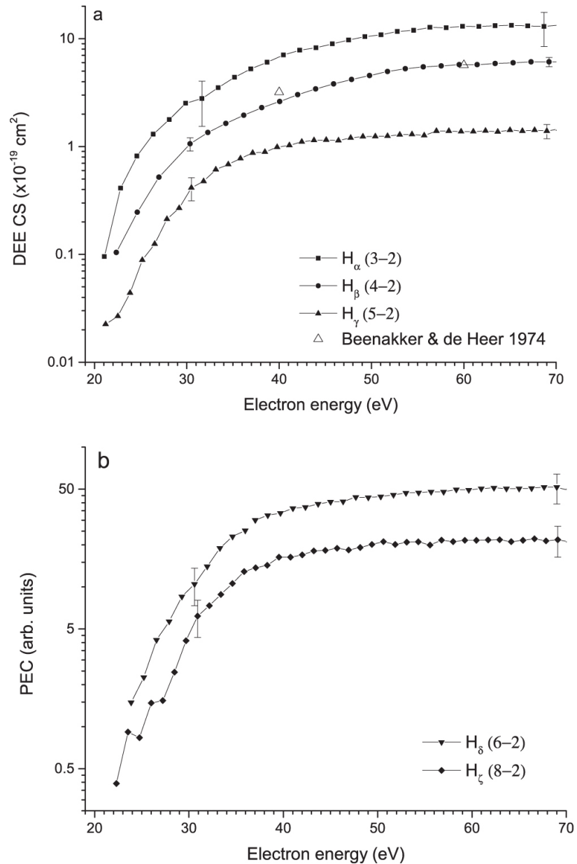
Figure 5. from Dissociative Excitation of Acetylene Induced by Electron Impact: Excitation-emission Cross-sections null 2017 APJ 841 17 doi:10.3847/1538-4357/aa6e54 https://dx.doi.org/10.3847/1538-4357/aa6e54 © 2017. The American Astronomical Society. All rights reserved.
