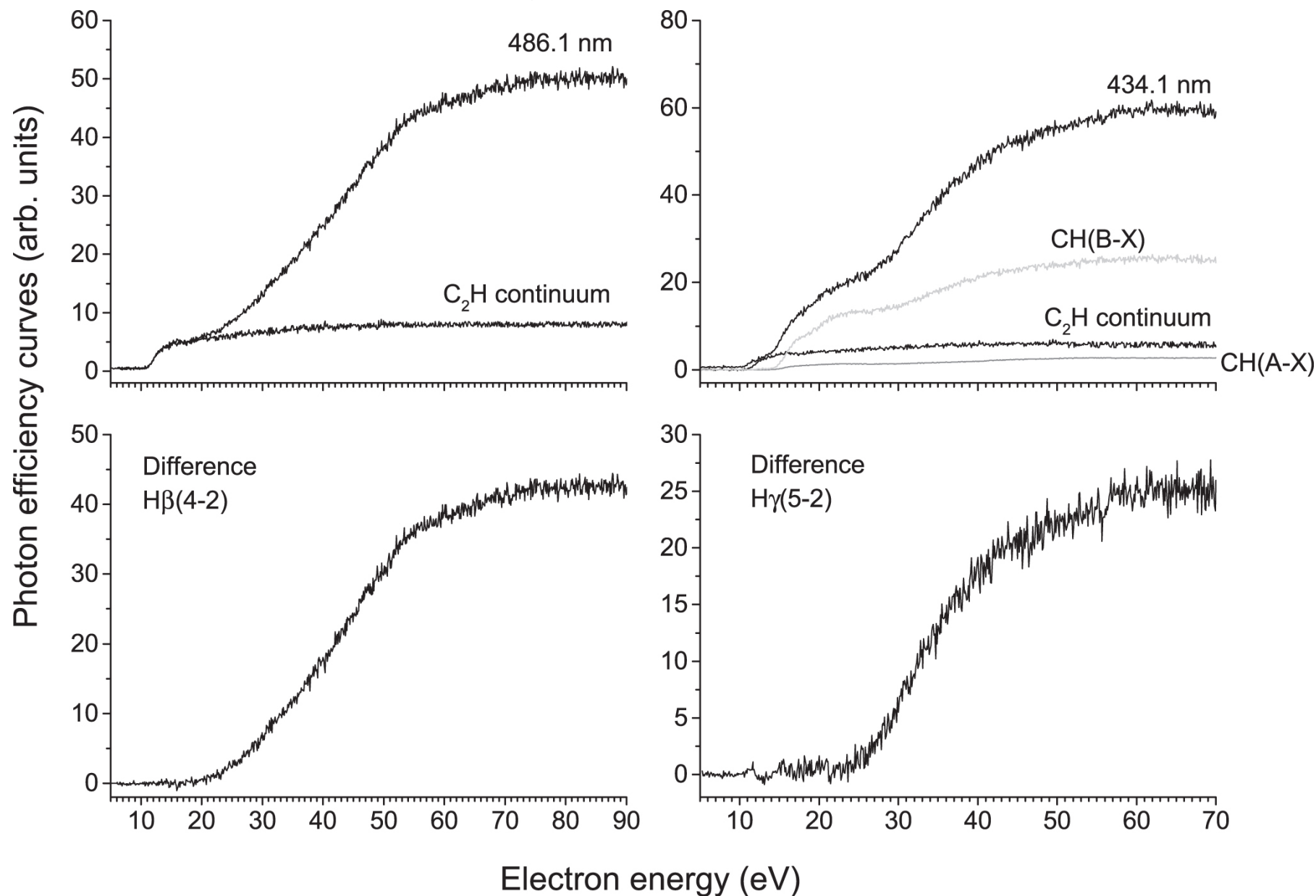
Figure 4. from Dissociative Excitation of Acetylene Induced by Electron Impact: Excitation-emission Cross-sections null 2017 APJ 841 17 doi:10.3847/1538-4357/aa6e54 https://dx.doi.org/10.3847/1538-4357/aa6e54
