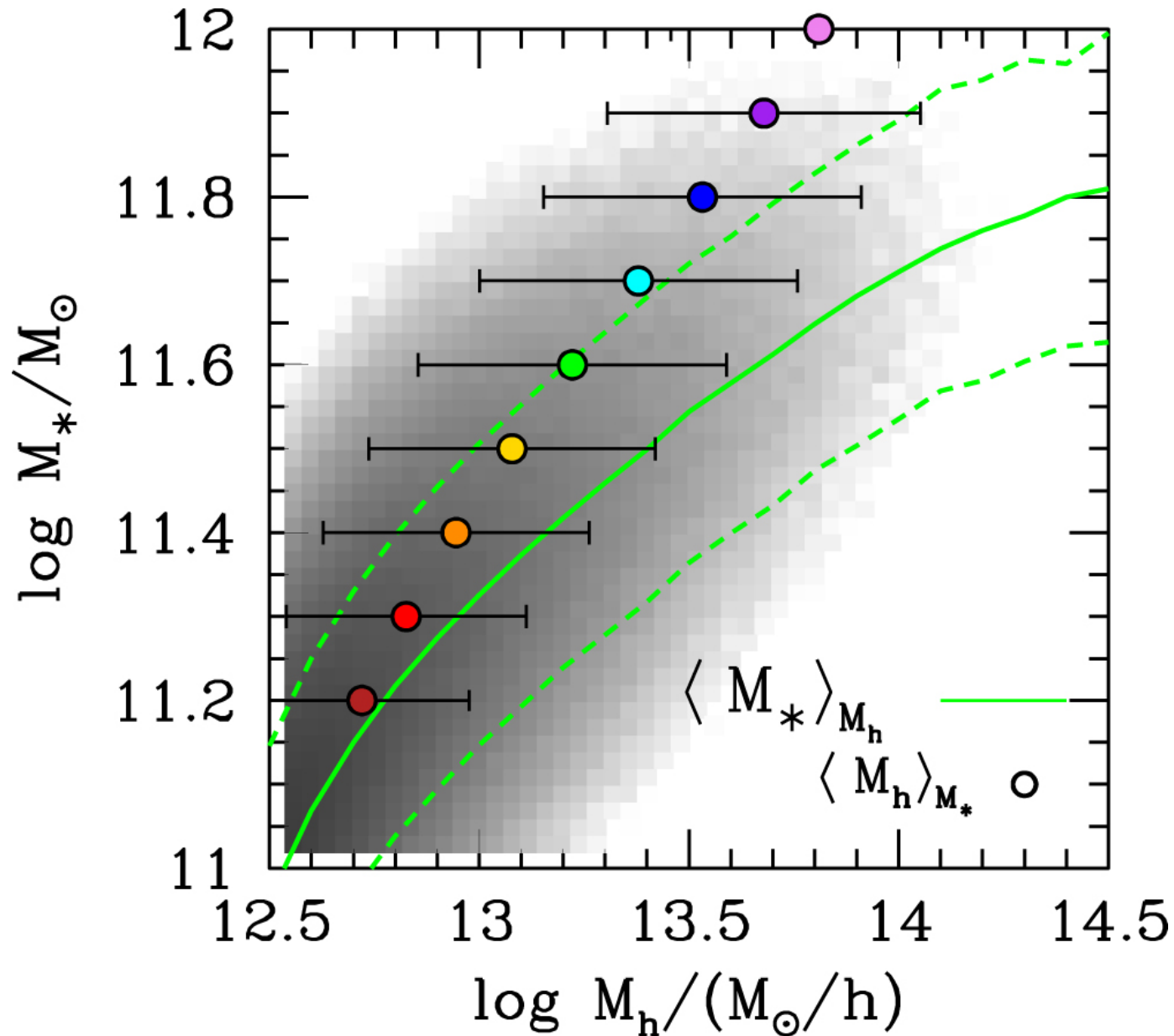
Figure 9. from The Correlation between Halo Mass and Stellar Mass for the Most Massive Galaxies in the Universe null 2017 APJ 839 121 doi:10.3847/1538-4357/aa6845 https://dx.doi.org/10.3847/1538-4357/aa6845 © 2017. The American Astronomical Society. All rights reserved.
