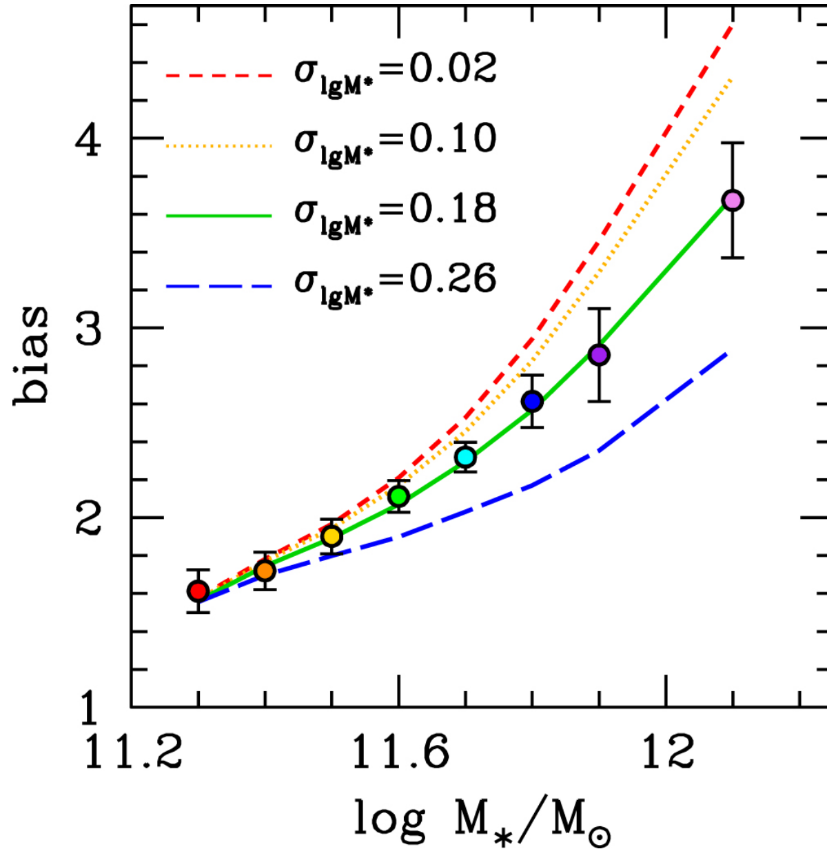
Figure 8. from The Correlation between Halo Mass and Stellar Mass for the Most Massive Galaxies in the Universe null 2017 APJ 839 121 doi:10.3847/1538-4357/aa6845 https://dx.doi.org/10.3847/1538-4357/aa6845 © 2017. The American Astronomical Society. All rights reserved.
