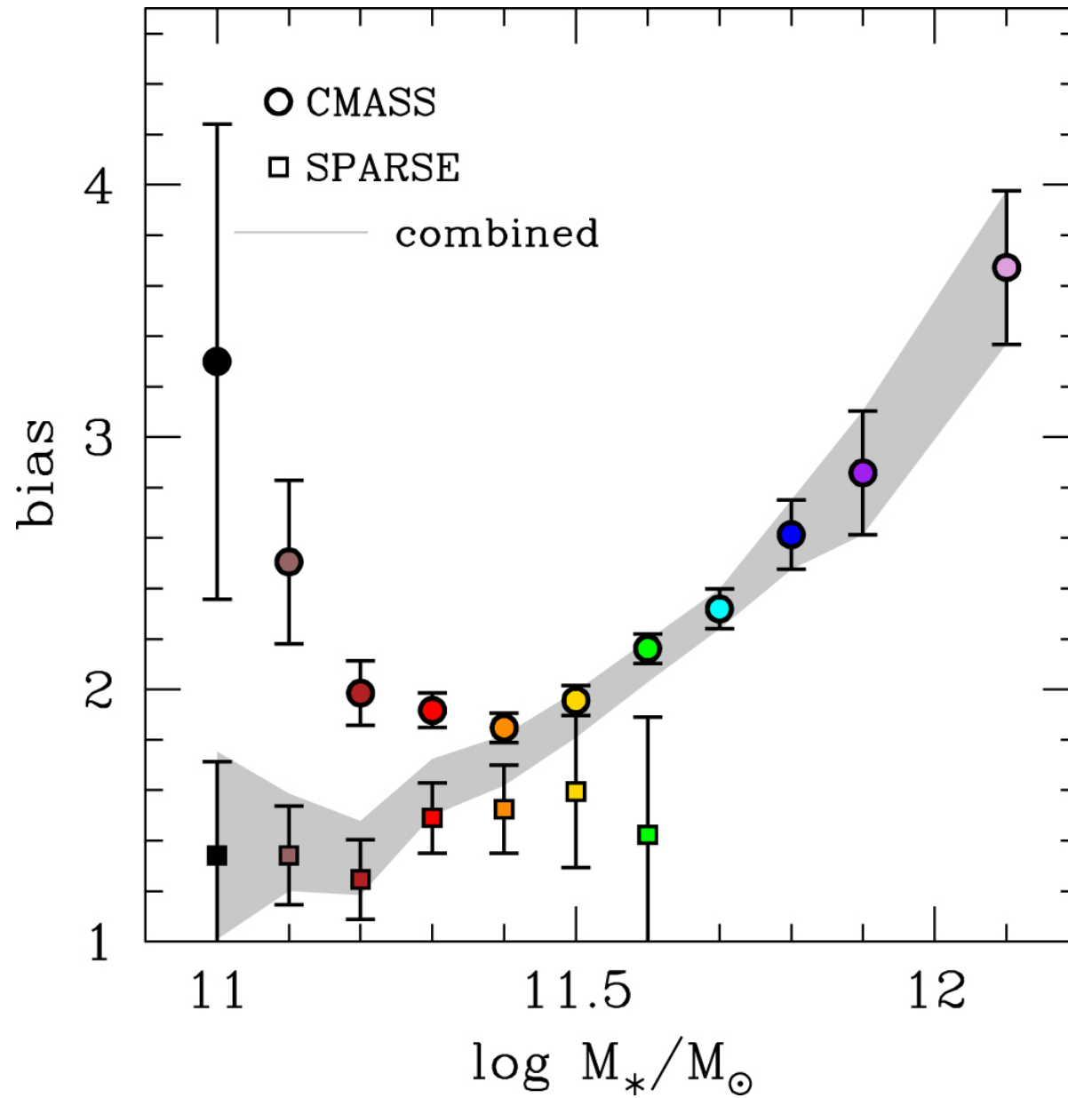
Figure 7. from The Correlation between Halo Mass and Stellar Mass for the Most Massive Galaxies in the Universe null 2017 APJ 839 121 doi:10.3847/1538-4357/aa6845 https://dx.doi.org/10.3847/1538-4357/aa6845 © 2017. The American Astronomical Society. All rights reserved.
