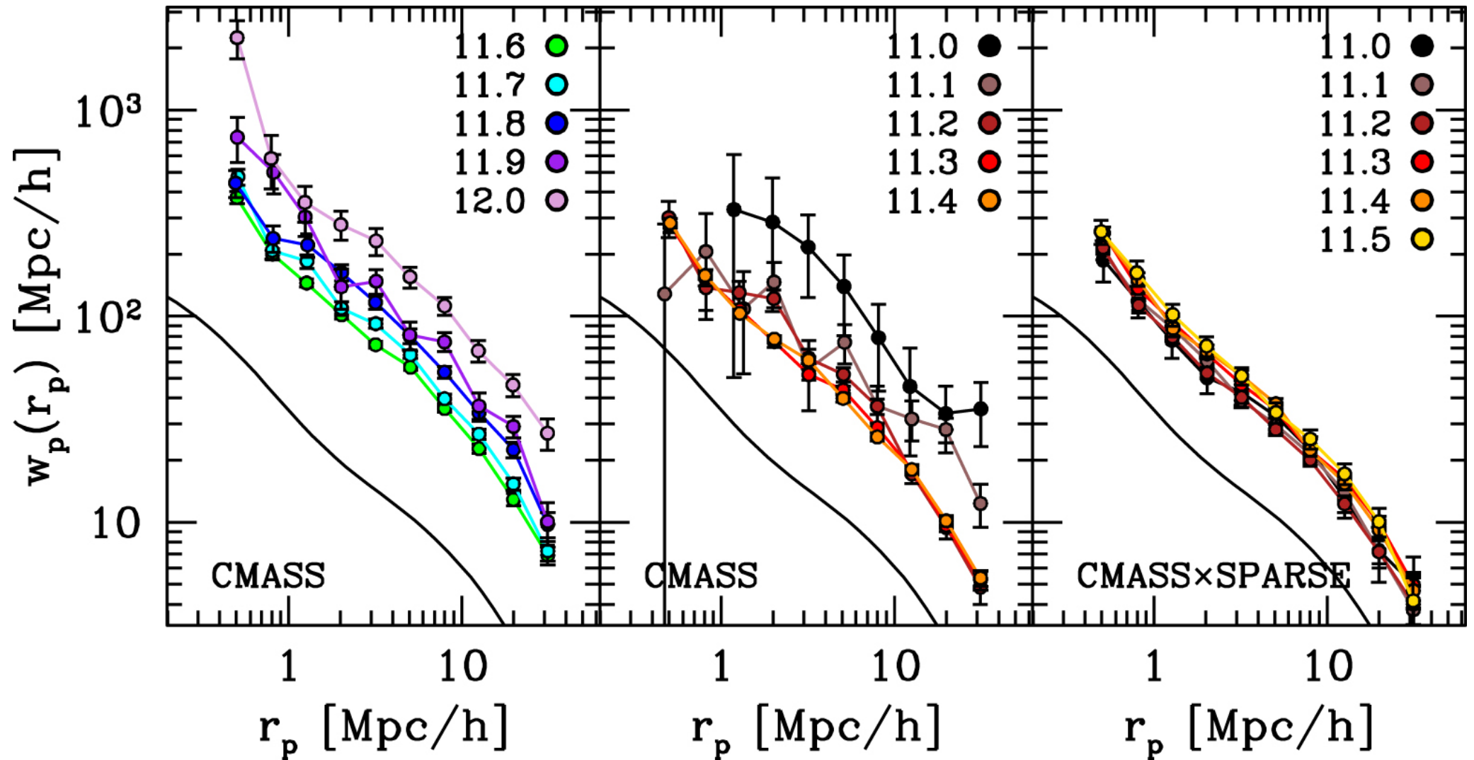
Figure 6. from The Correlation between Halo Mass and Stellar Mass for the Most Massive Galaxies in the Universe null 2017 APJ 839 121 doi:10.3847/1538-4357/aa6845 https://dx.doi.org/10.3847/1538-4357/aa6845 © 2017. The American Astronomical Society. All rights reserved.
