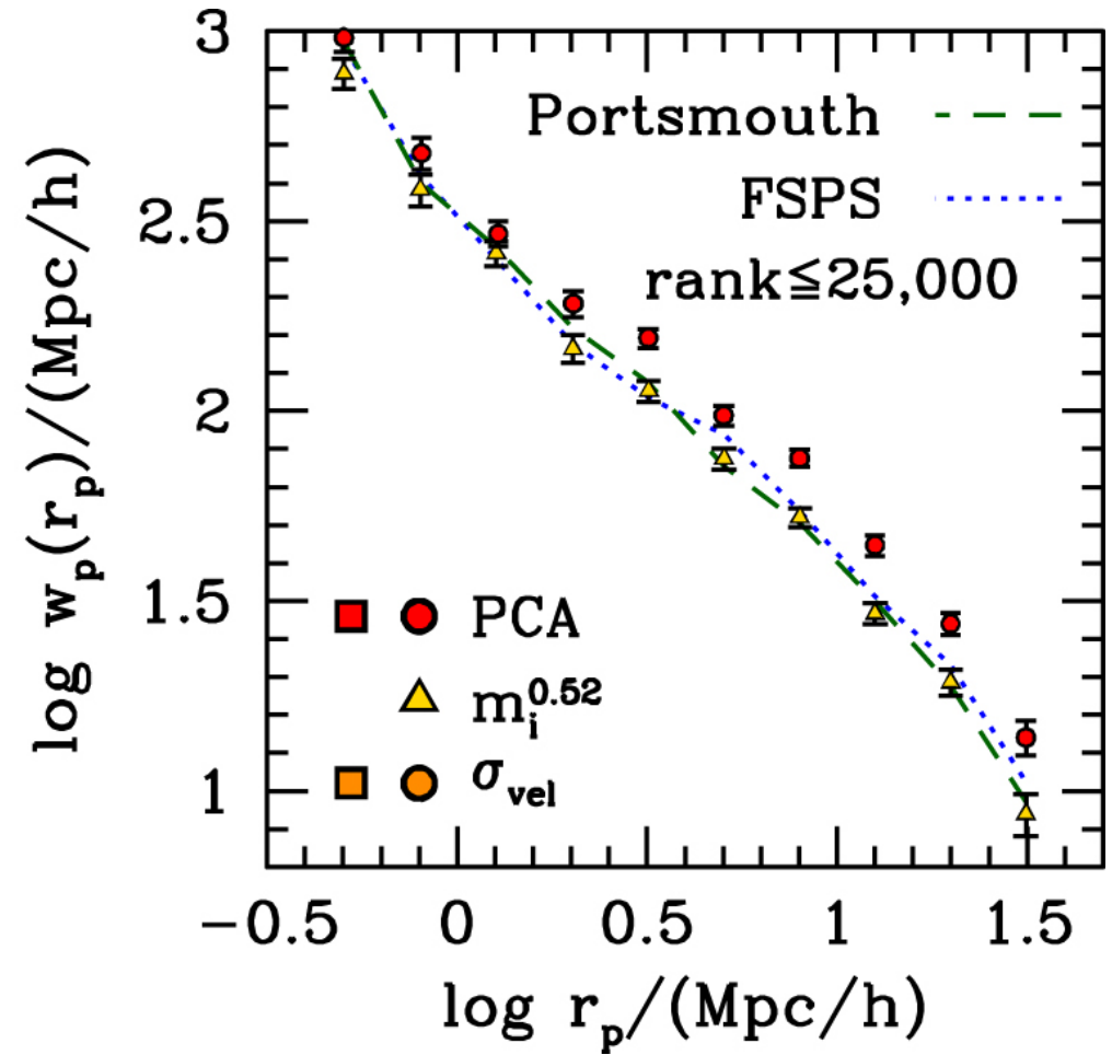
Figure 5. from The Correlation between Halo Mass and Stellar Mass for the Most Massive Galaxies in the Universe null 2017 APJ 839 121 doi:10.3847/1538-4357/aa6845 https://dx.doi.org/10.3847/1538-4357/aa6845 © 2017. The American Astronomical Society. All rights reserved.
