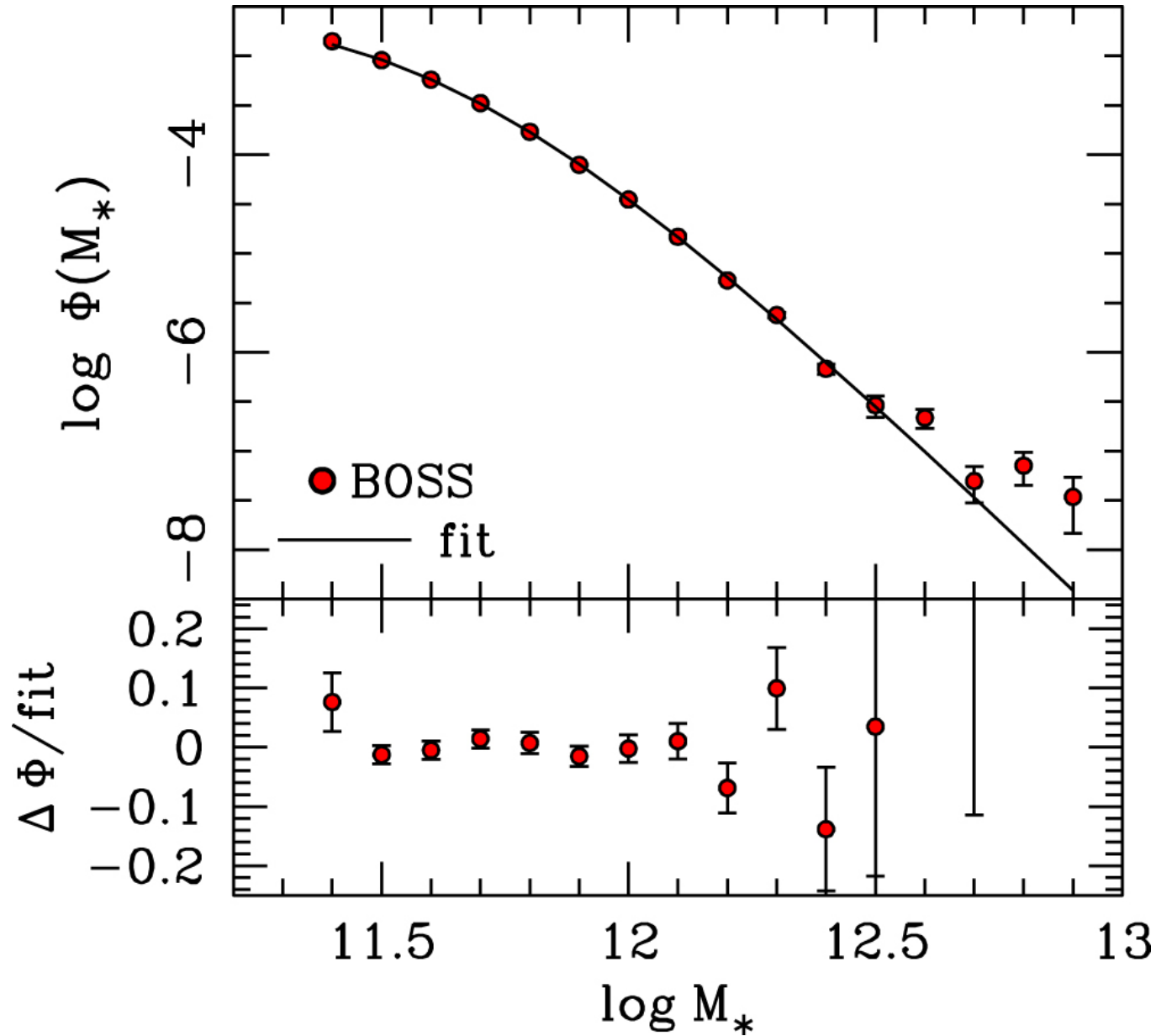
Figure 4. from The Correlation between Halo Mass and Stellar Mass for the Most Massive Galaxies in the Universe null 2017 APJ 839 121 doi:10.3847/1538-4357/aa6845 https://dx.doi.org/10.3847/1538-4357/aa6845 © 2017. The American Astronomical Society. All rights reserved.
