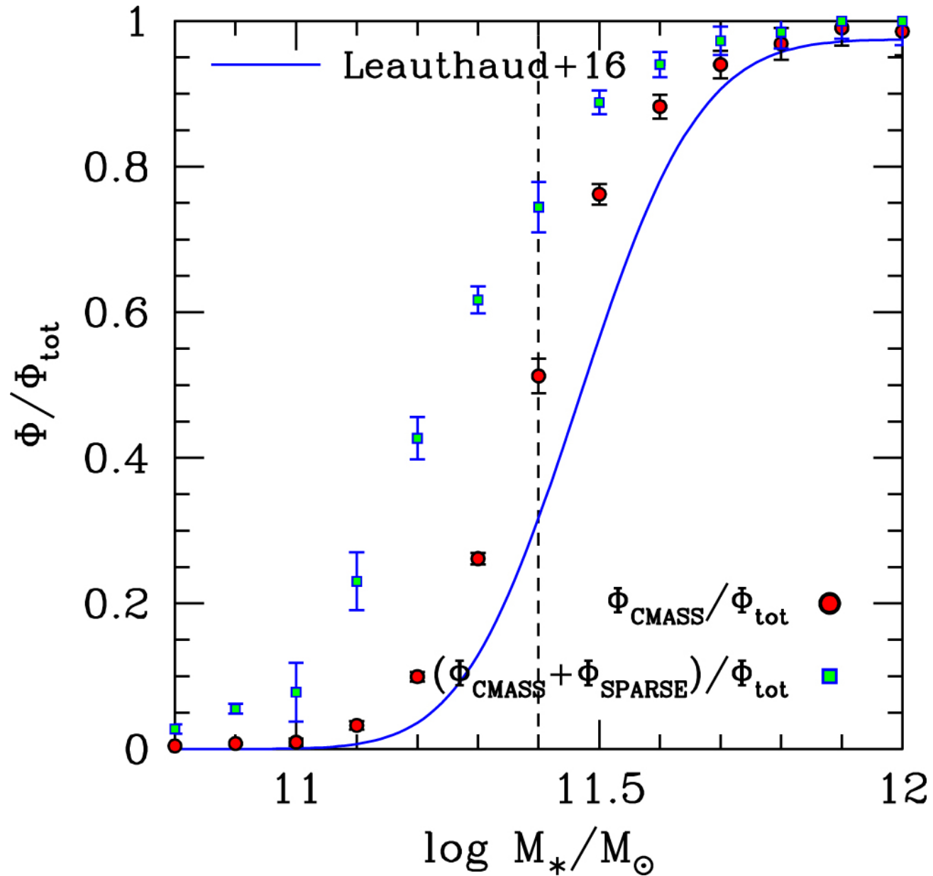
Figure 3. from The Correlation between Halo Mass and Stellar Mass for the Most Massive Galaxies in the Universe null 2017 APJ 839 121 doi:10.3847/1538-4357/aa6845 https://dx.doi.org/10.3847/1538-4357/aa6845 © 2017. The American Astronomical Society. All rights reserved.
