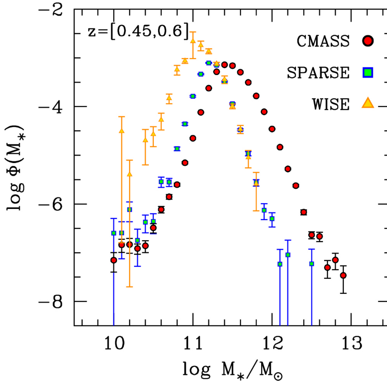
Figure 2. from The Correlation between Halo Mass and Stellar Mass for the Most Massive Galaxies in the Universe null 2017 APJ 839 121 doi:10.3847/1538-4357/aa6845 https://dx.doi.org/10.3847/1538-4357/aa6845 © 2017. The American Astronomical Society. All rights reserved.
