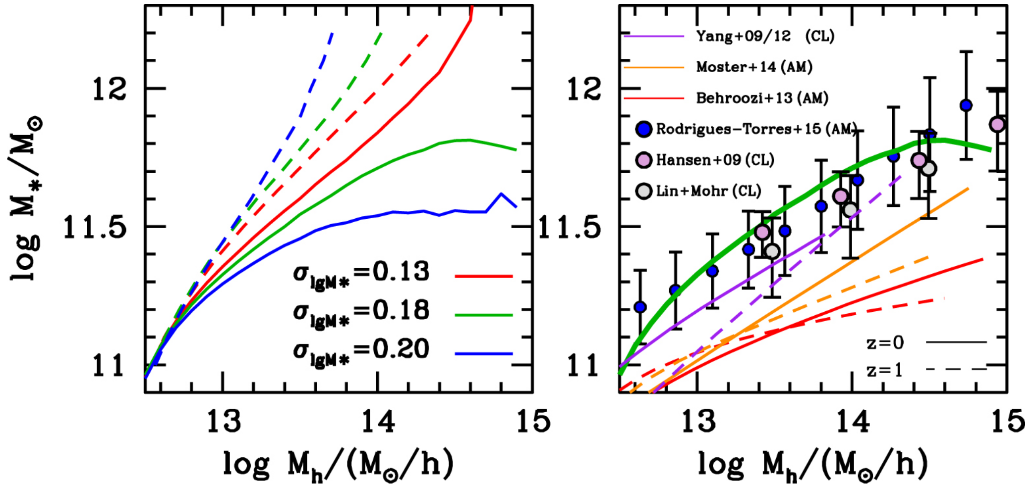
Figure 10. from The Correlation between Halo Mass and Stellar Mass for the Most Massive Galaxies in the Universe null 2017 APJ 839 121 doi:10.3847/1538-4357/aa6845 https://dx.doi.org/10.3847/1538-4357/aa6845 © 2017. The American Astronomical Society. All rights reserved.
