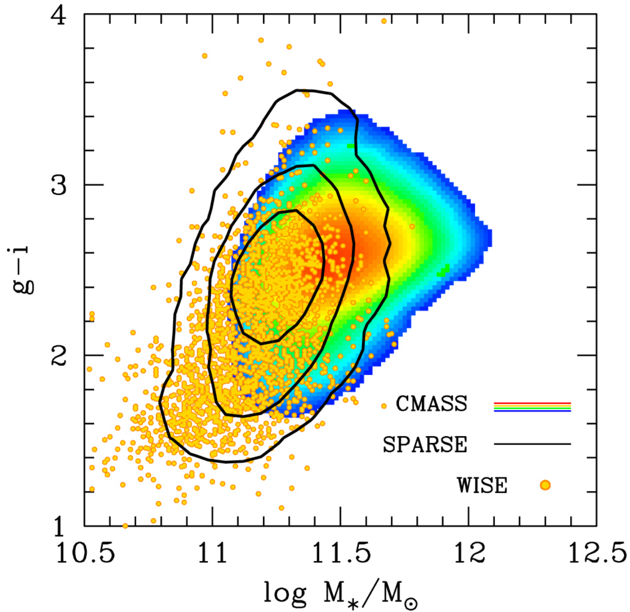
Figure 1. from The Correlation between Halo Mass and Stellar Mass for the Most Massive Galaxies in the Universe null 2017 APJ 839 121 doi:10.3847/1538-4357/aa6845 https://dx.doi.org/10.3847/1538-4357/aa6845 © 2017. The American Astronomical Society. All rights reserved.
