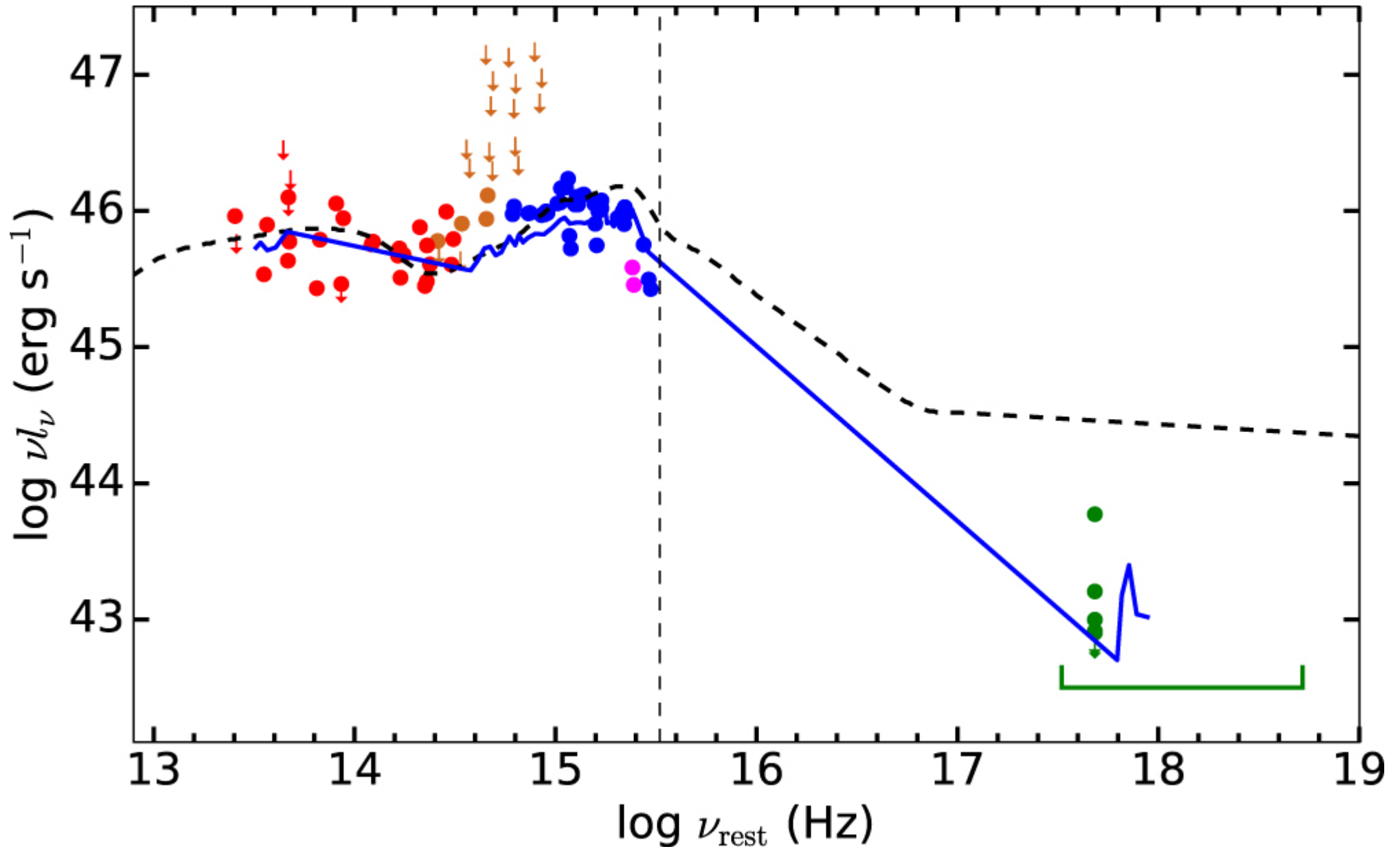
Figure 5. from X-Ray Insights into the Nature of Quasars with Redshifted Broad Absorption Lines null 2017 APJ 839 101 doi:10.3847/1538-4357/aa6842 https://dx.doi.org/10.3847/1538-4357/aa6842 © 2017. The American Astronomical Society. All rights reserved.
