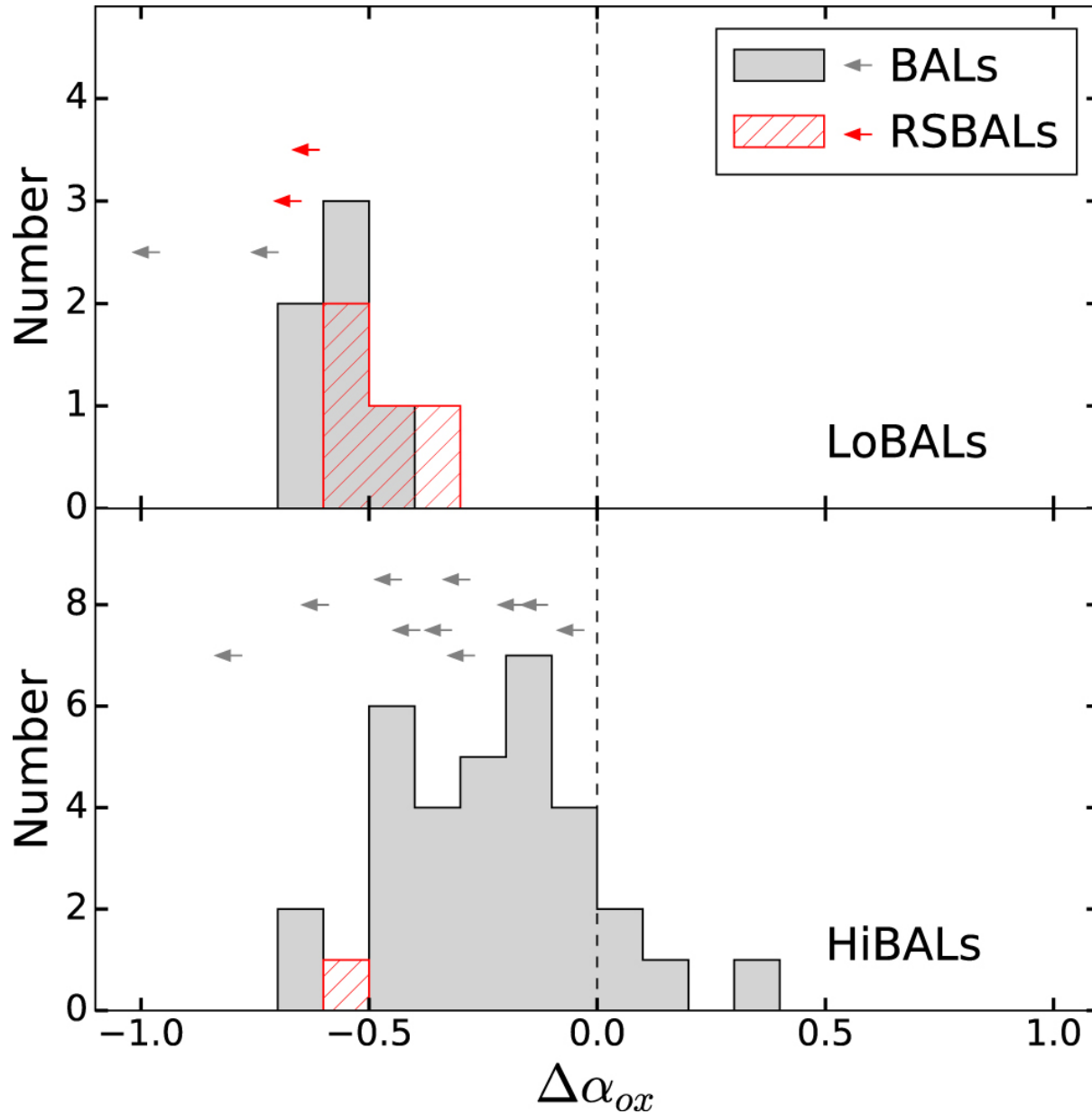
Figure 4. from X-Ray Insights into the Nature of Quasars with Redshifted Broad Absorption Lines null 2017 APJ 839 101 doi:10.3847/1538-4357/aa6842 https://dx.doi.org/10.3847/1538-4357/aa6842 © 2017. The American Astronomical Society. All rights reserved.
