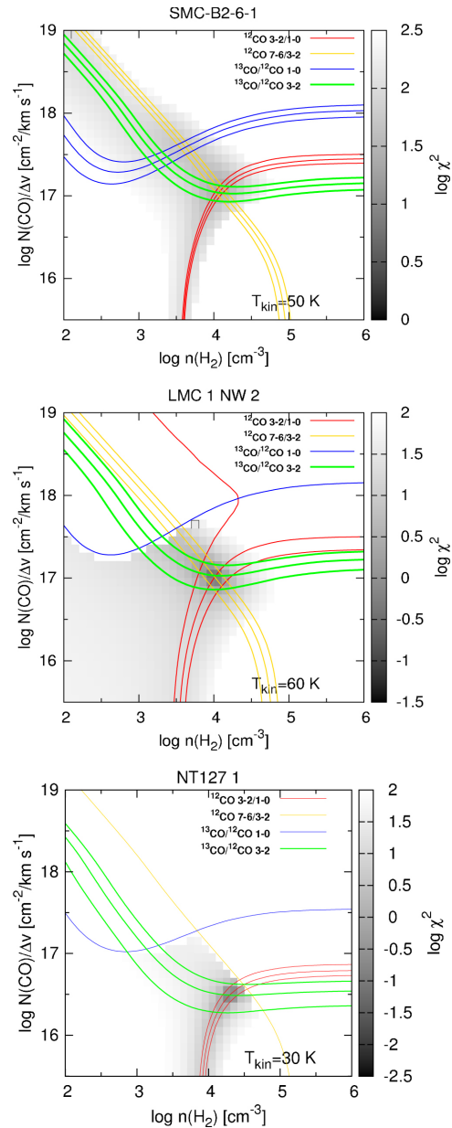
Figure 9. from Characterizing the Transition from Diffuse Atomic to Dense Molecular Clouds in the Magellanic Clouds with [C II], [C I], and CO null 2017 APJ 839 107 doi:10.3847/1538-4357/aa683a https://dx.doi.org/10.3847/1538-4357/aa683a © 2017. The American Astronomical Society. All rights reserved.
