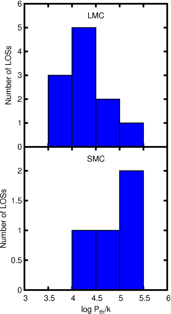
Figure 8. from Characterizing the Transition from Diffuse Atomic to Dense Molecular Clouds in the Magellanic Clouds with [C II], [C I], and CO null 2017 APJ 839 107 doi:10.3847/1538-4357/aa683a https://dx.doi.org/10.3847/1538-4357/aa683a © 2017. The American Astronomical Society. All rights reserved.
