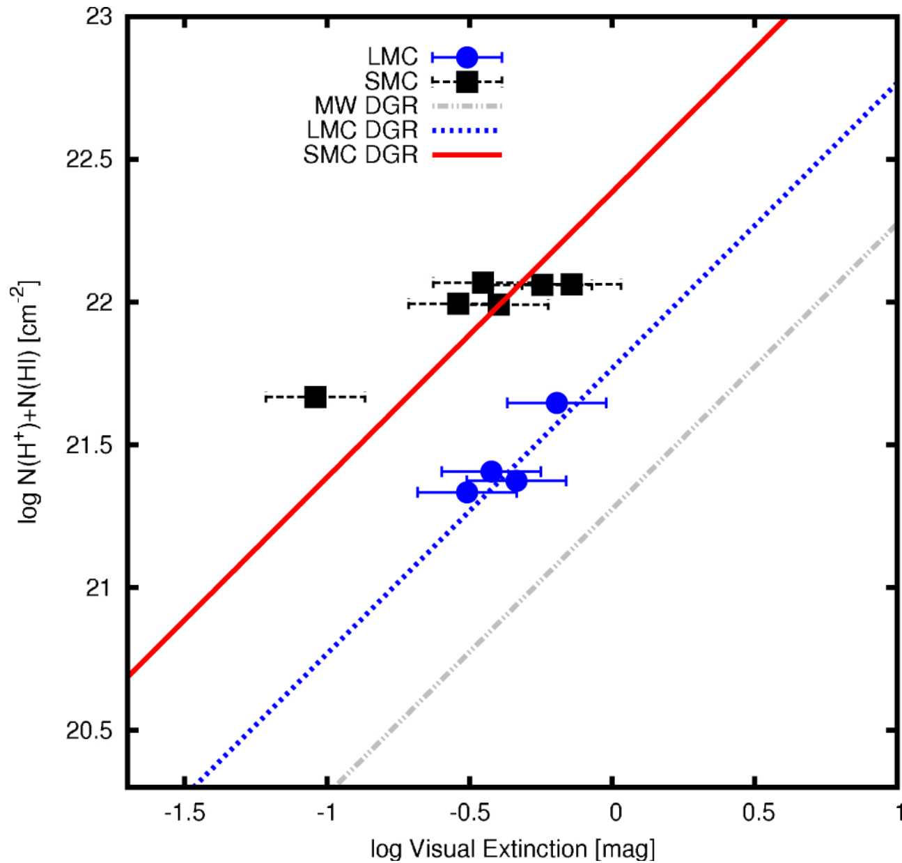
Figure 7. from Characterizing the Transition from Diffuse Atomic to Dense Molecular Clouds in the Magellanic Clouds with [C II], [C I], and CO null 2017 APJ 839 107 doi:10.3847/1538-4357/aa683a https://dx.doi.org/10.3847/1538-4357/aa683a © 2017. The American Astronomical Society. All rights reserved.
