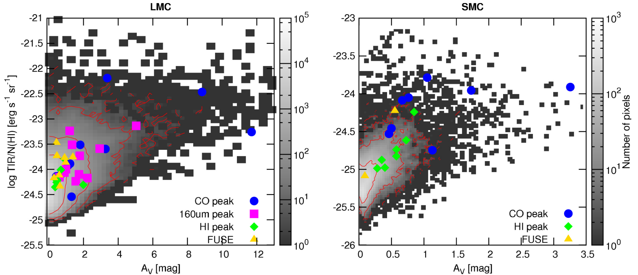
Figure 3. from Characterizing the Transition from Diffuse Atomic to Dense Molecular Clouds in the Magellanic Clouds with [C II], [C I], and CO null 2017 APJ 839 107 doi:10.3847/1538-4357/aa683a https://dx.doi.org/10.3847/1538-4357/aa683a © 2017. The American Astronomical Society. All rights reserved.
