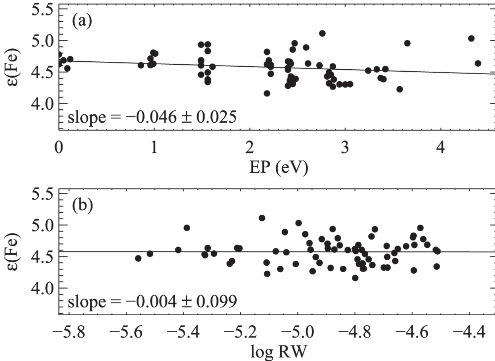
Figure 9. from Triangulum II. Not Especially Dense After All null 2017 APJ 838 83 doi:10.3847/1538-4357/aa6570 https://dx.doi.org/10.3847/1538-4357/aa6570 © 2017. The American Astronomical Society. All rights reserved.
