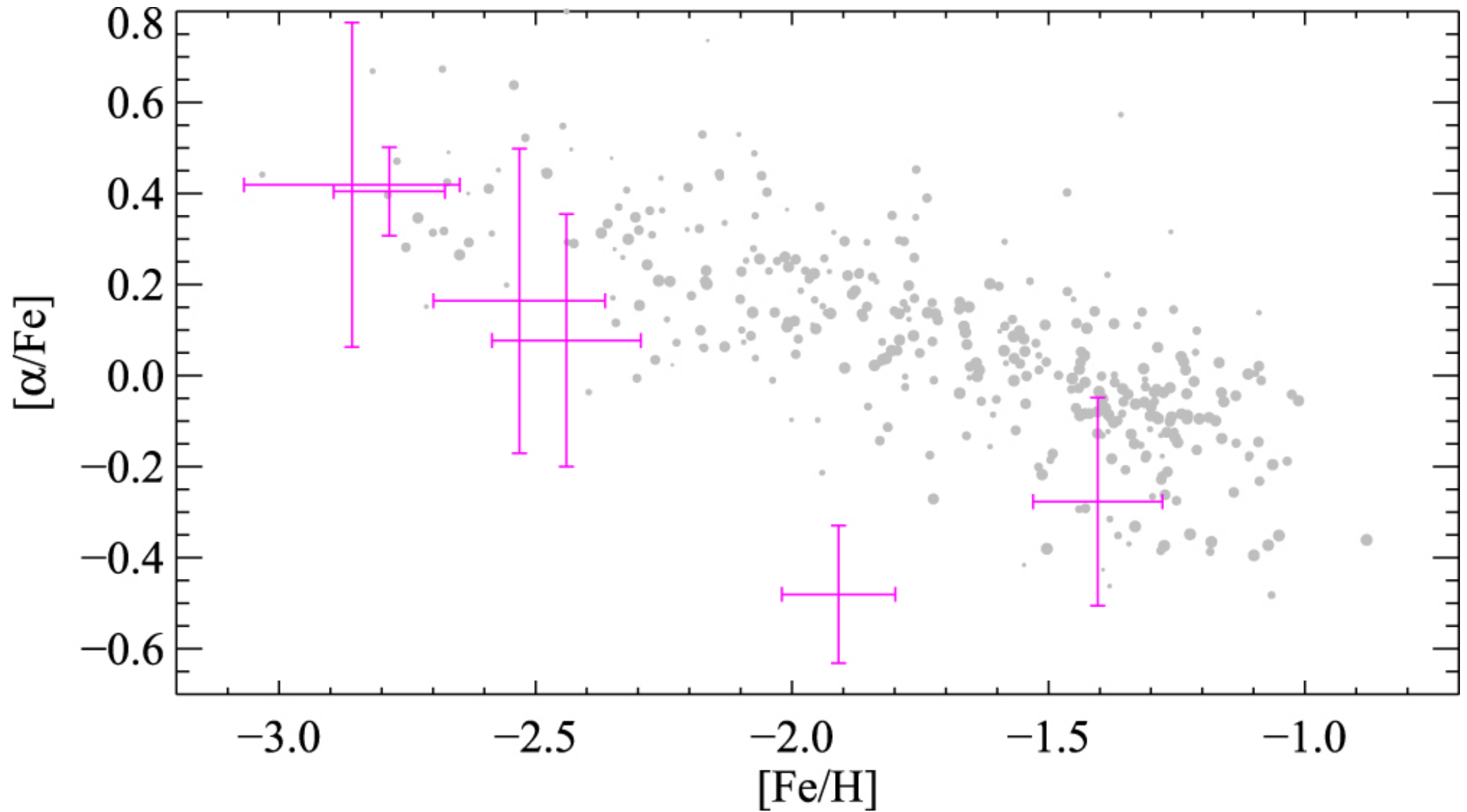
Figure 8. from Triangulum II. Not Especially Dense After All null 2017 APJ 838 83 doi:10.3847/1538-4357/aa6570 https://dx.doi.org/10.3847/1538-4357/aa6570 © 2017. The American Astronomical Society. All rights reserved.
